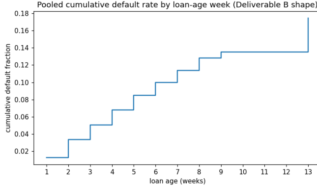
Figure 2: Pooled cumulative default rate by loan-age week: a concave rise through week 9, a flat stretch (weeks 9–12), and the day-90 open-balance cliff at week 13. Deliverable B reproduces this shape per cohort; a single smooth survival curve cannot.
