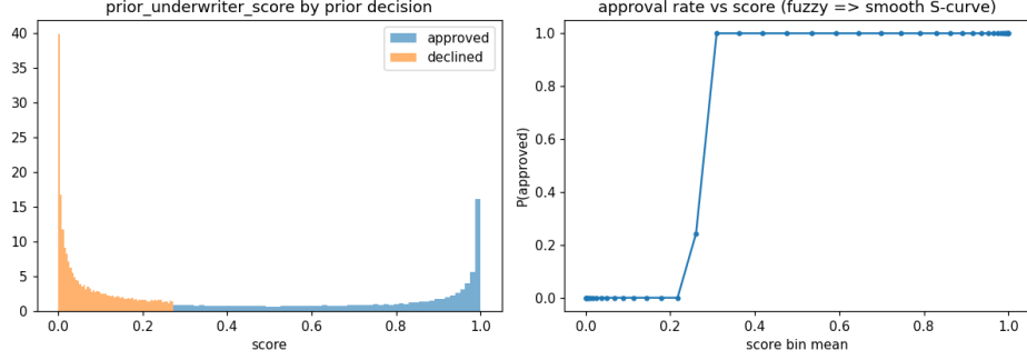
Figure 1: The prior lender’s approval rule is a sharp threshold at prior_underwriter_score = 0.273 . The approved and declined score distributions do not overlap (left), and the approval rate is a step function of the score (right); labels are observed only to the right of the cut. This is the source of the selection bias and the reason inverse-propensity reweighting is infeasible.
