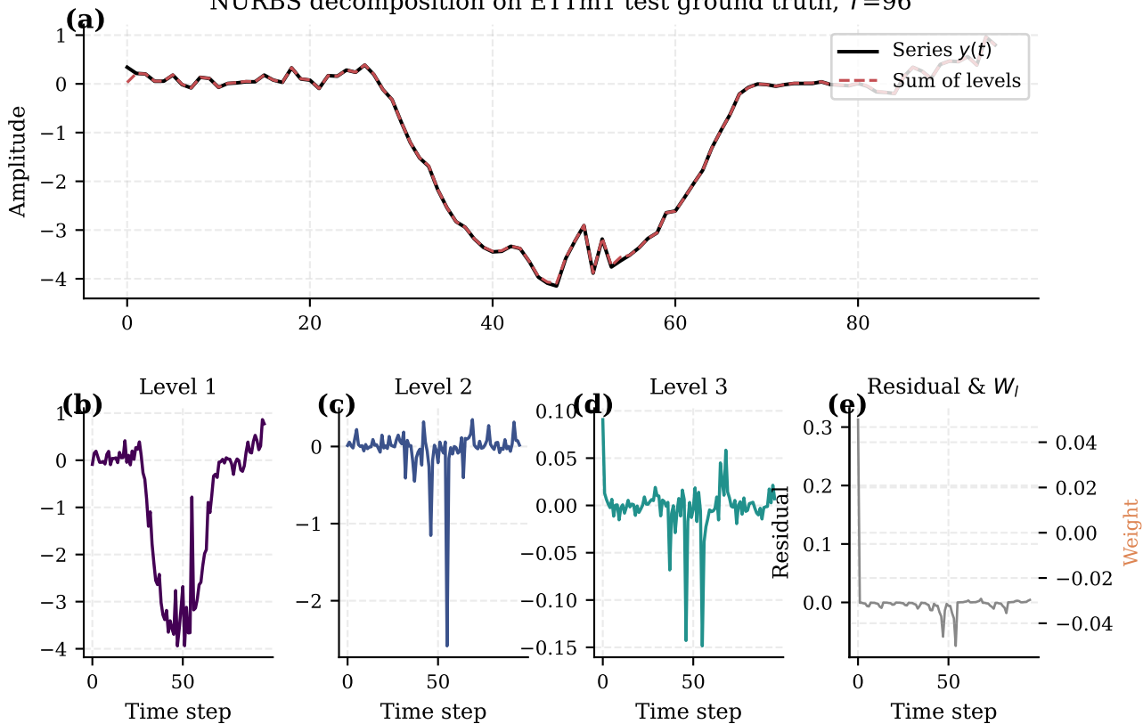
NURBS decomposition on ETTm1 test ground truth, T=96
