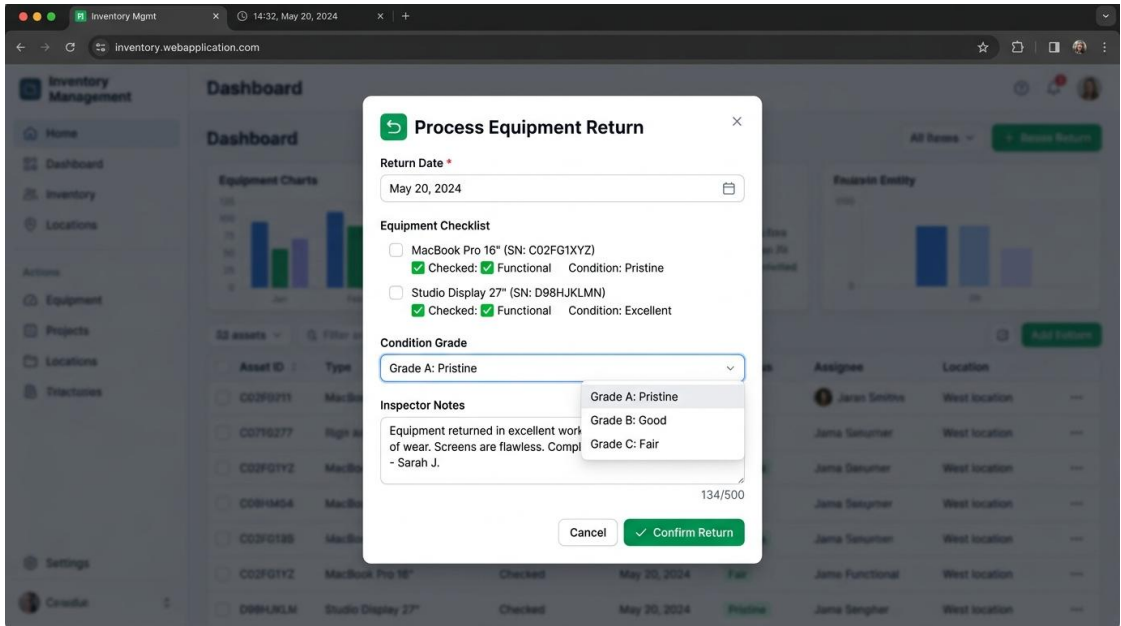
Figure 2: Verified Process Equipment Return inspection modal dialog with condition grade checklist and inspector notes.
