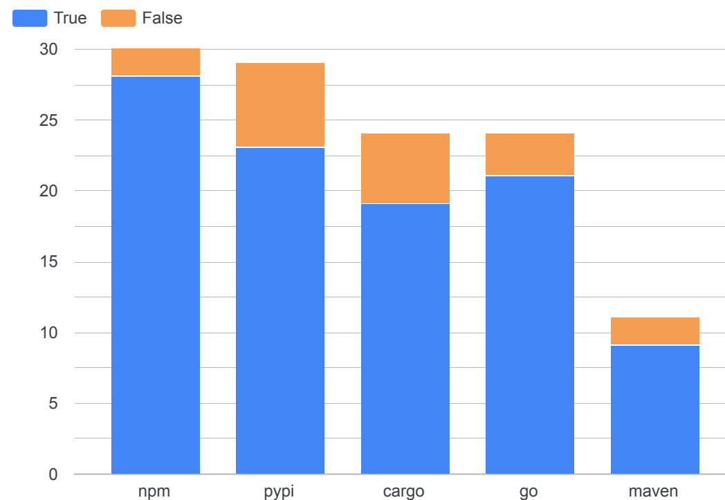
Decision Pass Rate by Package Ecosystem
