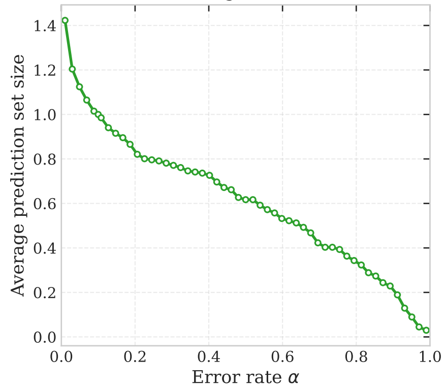
Average set size
