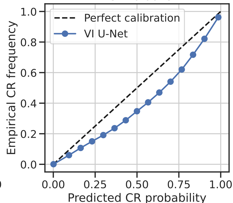
F814W - Resolved Galaxies ECE=0.0019
