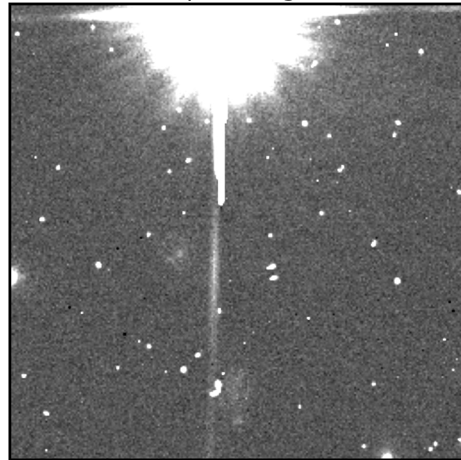
Input Image
