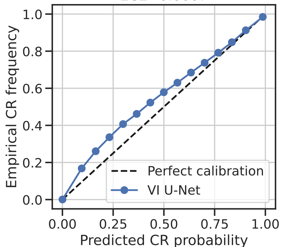
F606W - Globular Clusters ECE=0.0005
