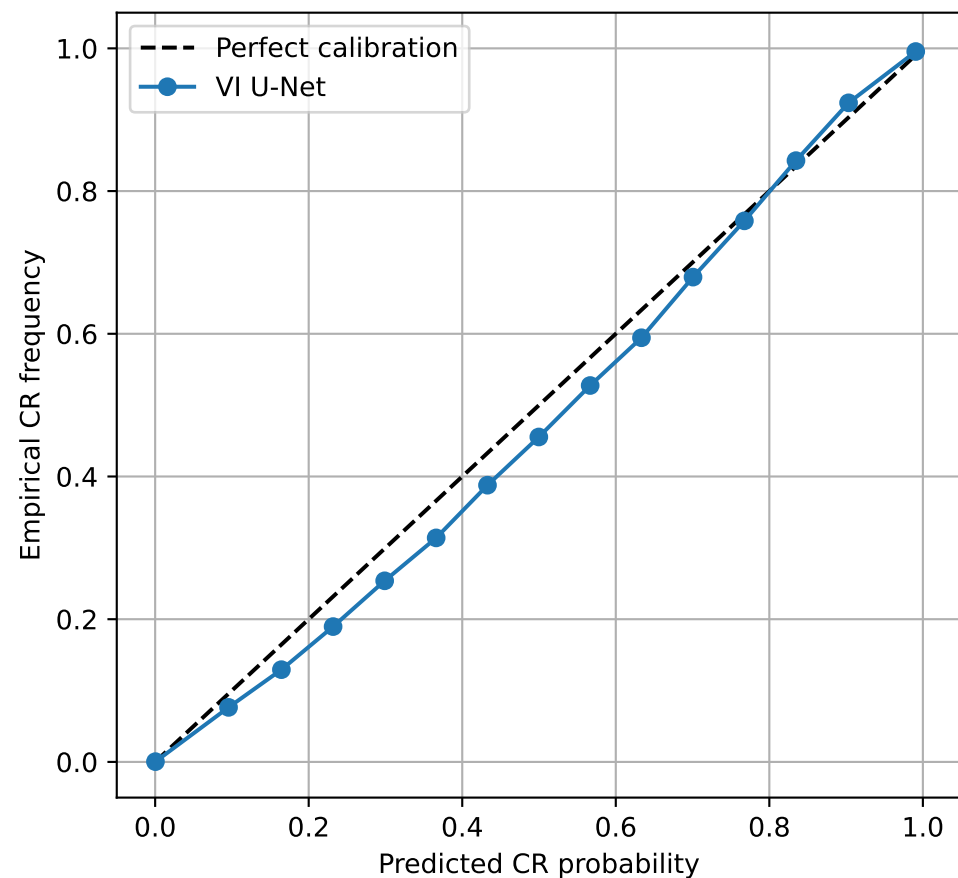
F814W - Globular Clusters ECE=0.0014
