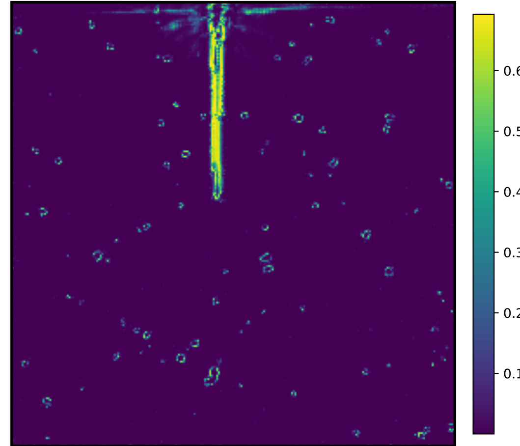
Uncertainty (Entropy)
