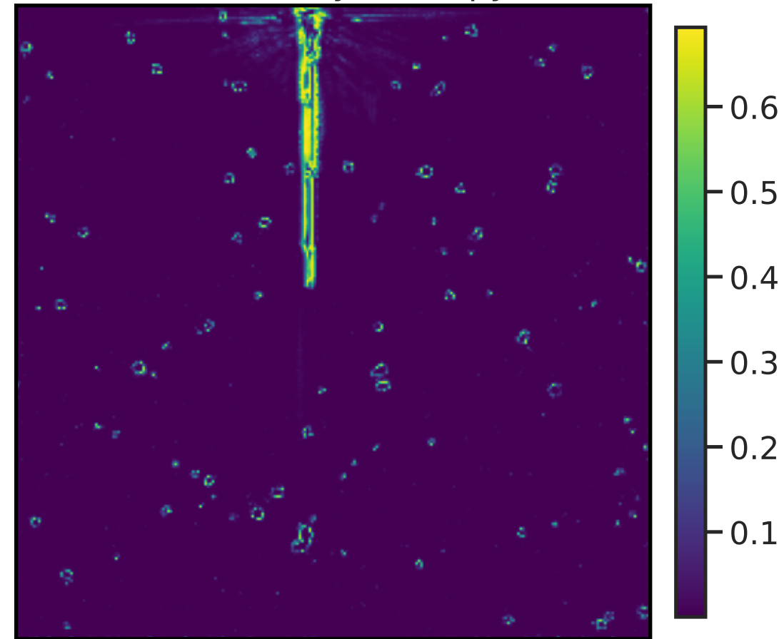
Uncertainty (Entropy)
