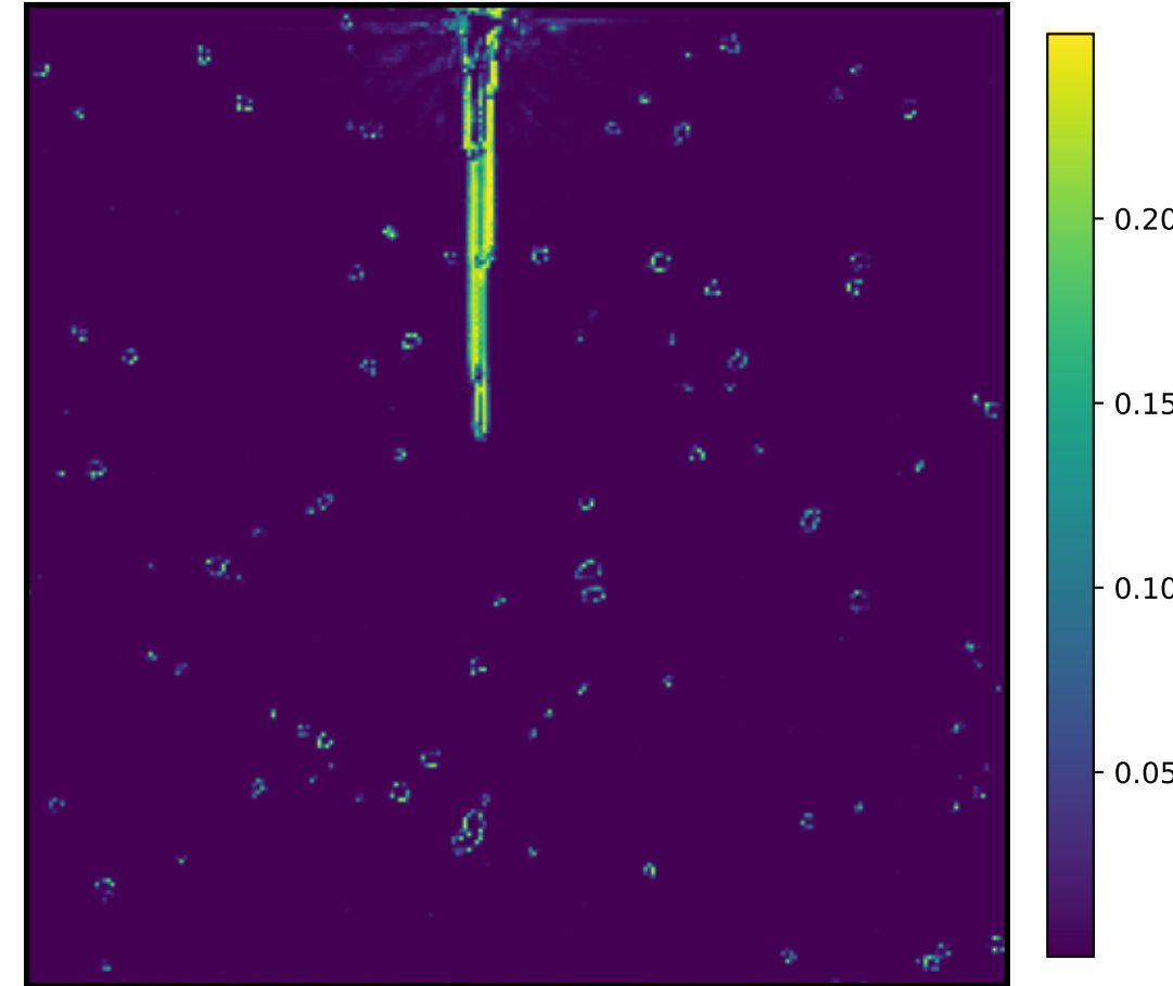
Uncertainty Proxy p(1-p)
