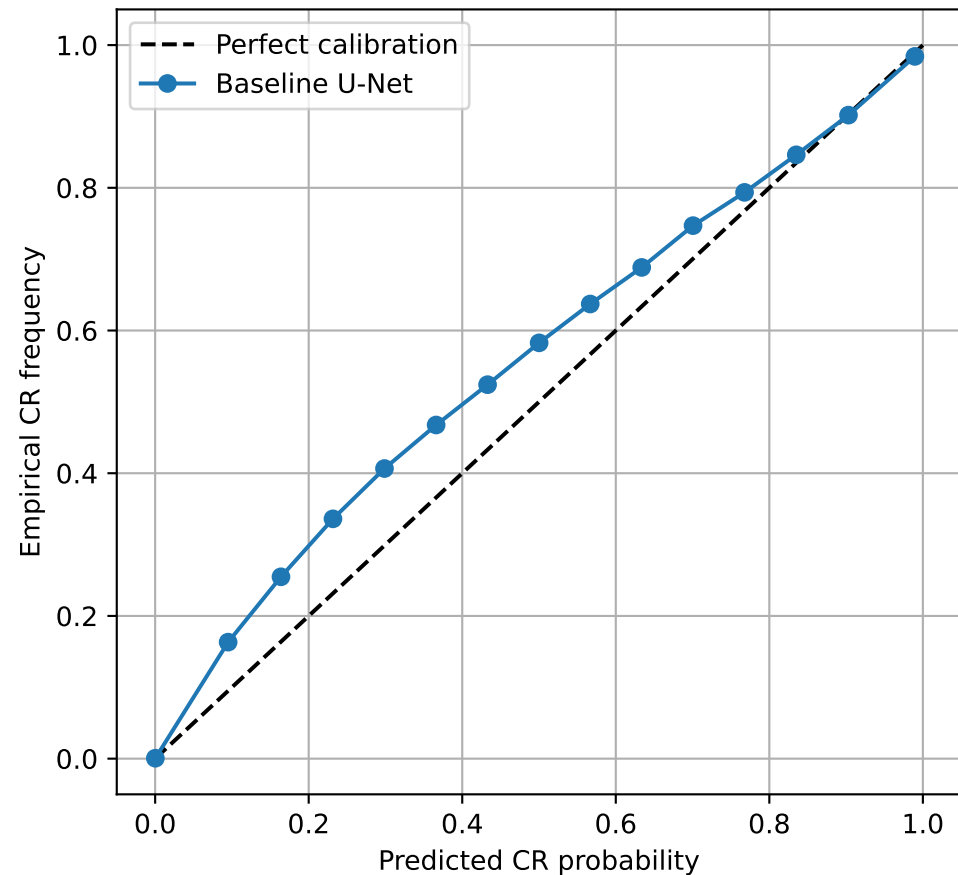
F606W - Globular Clusters ECE=0.0003
