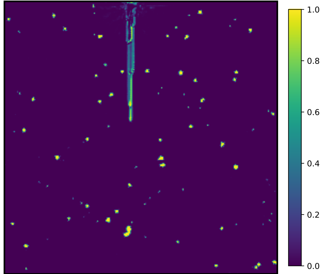
CR Probability Mask
