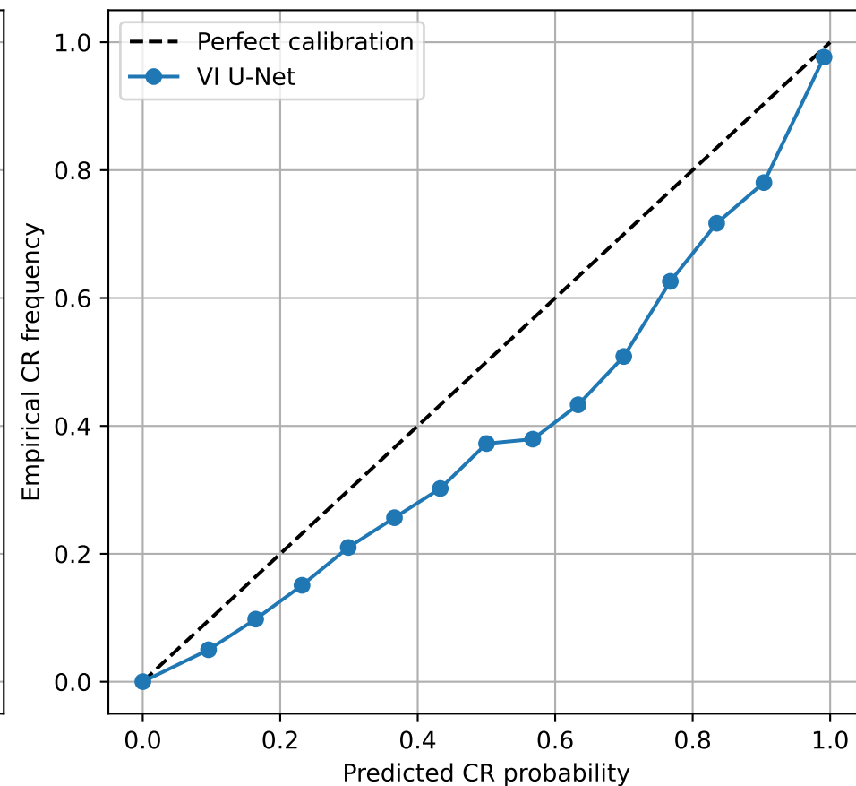
F606W - Extragalactic Fields ECE=0.0010
