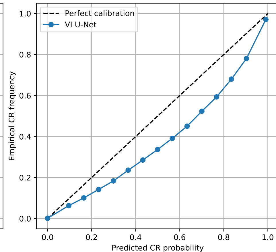
F606W - Resolved Galaxies ECE=0.0011
