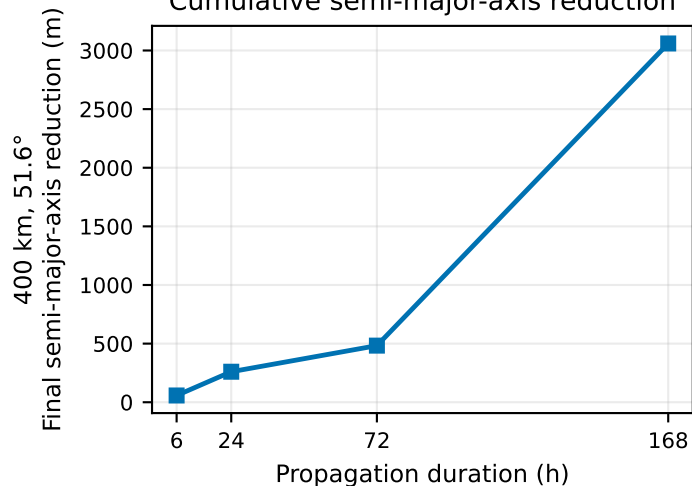
Cumulative semi-major-axis reduction
