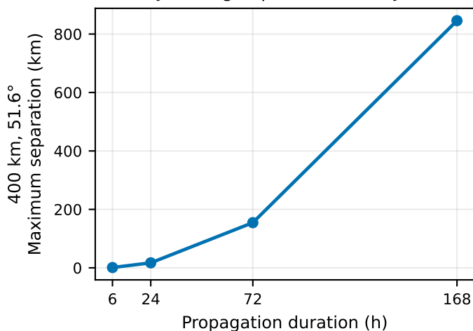
J2+drag separation from J2
