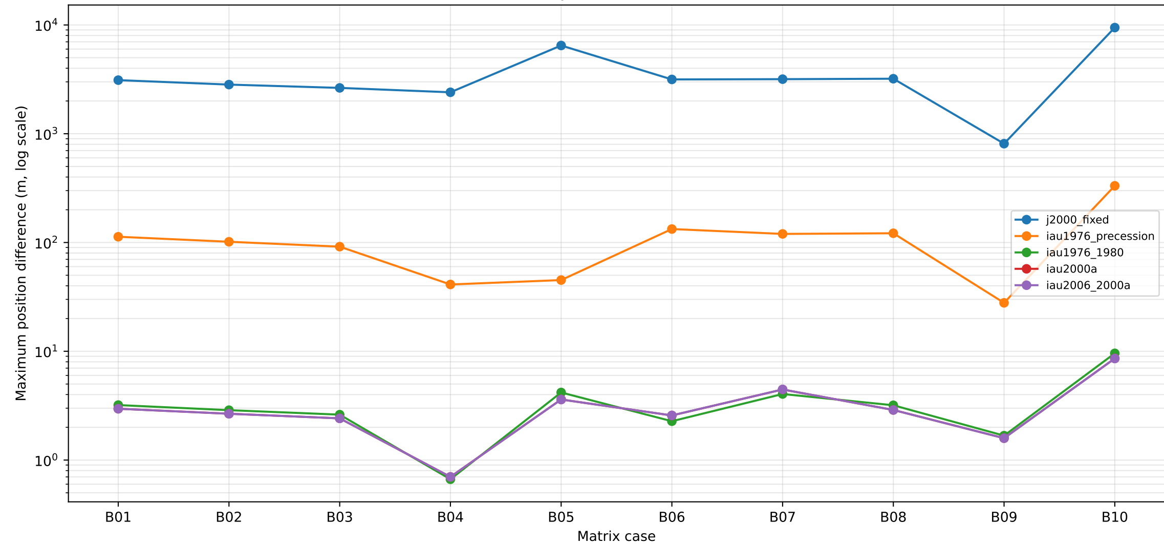
GMAT residual by Earth-orientation realization
