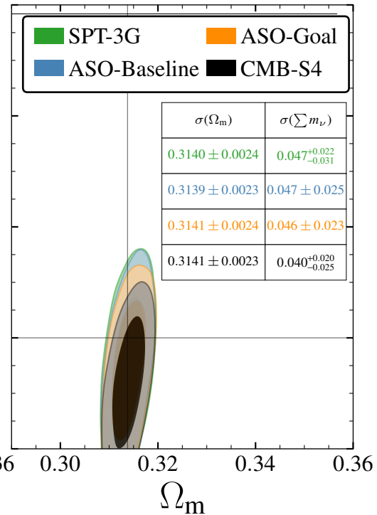
CMB+SNe+BAO
