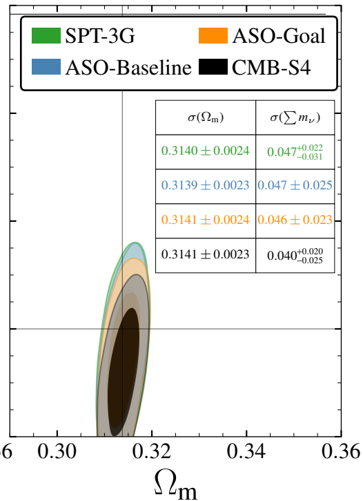
CMB+SNe+BAO
