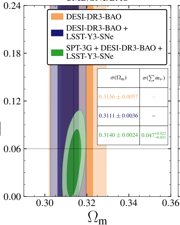
CMB/SNe/BAO
