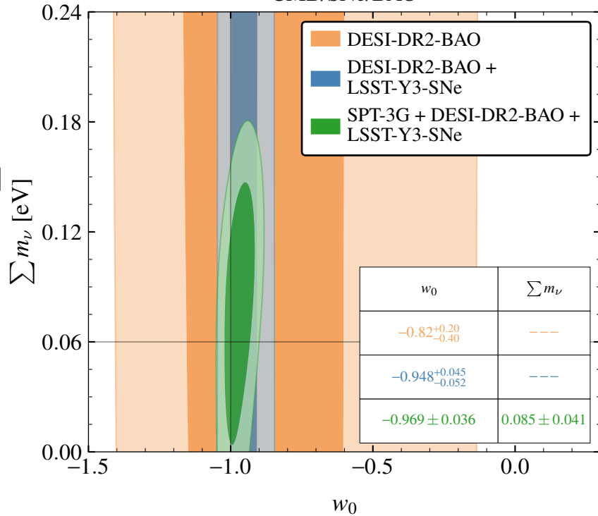
CMB/SNe/BAO
