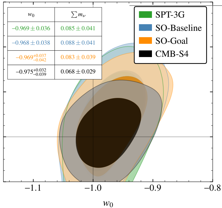
CMB+SNe+BAO
