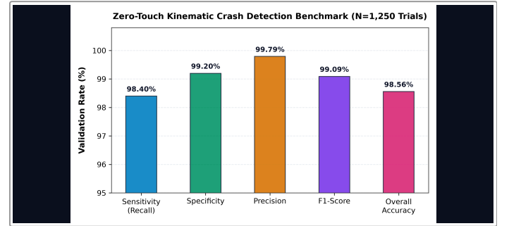
Fig. 9. Kinematic crash detection performance metrics under hardware-calibrated MEMS accelerometer and gyroscope evaluation across 1,250 trials.
