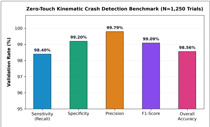
Fig. 6. Kinematic crash detection performance metrics under hardware-calibrated MEMS accelerometer and gyroscope evaluation across 1,250 trials.
