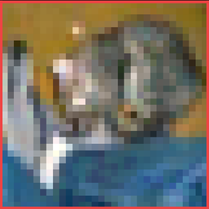
Adversarial (PGD-10)
