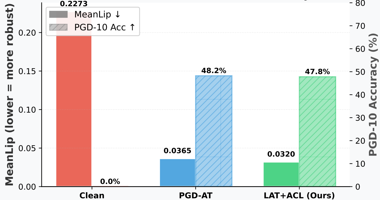
MeanLip vs PGD-10 Robustness (our metric vs actual attack accuracy)
