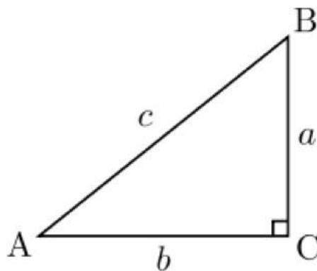
Figure 23.1: Right-angled triangle
