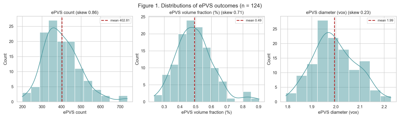
Figure 1. Distributions of the ePVS outcomes. Counts and volumes are right-skewed (log-transformed for testing); diameter is roughly normal.
