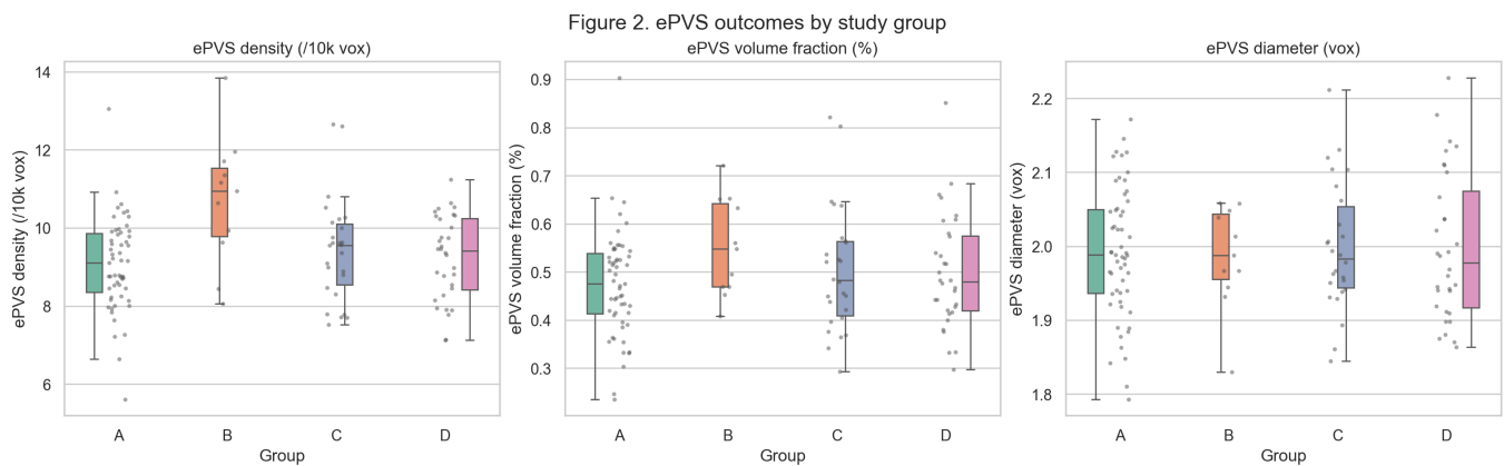
Figure 2. ePVS outcomes by group. Group B has the highest density; volume fraction and diameter look similar across groups.
