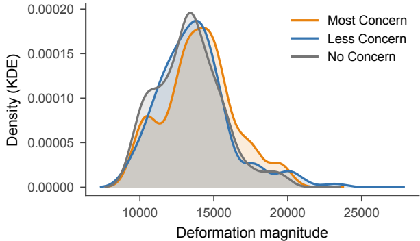
DILI class deformation distributions
