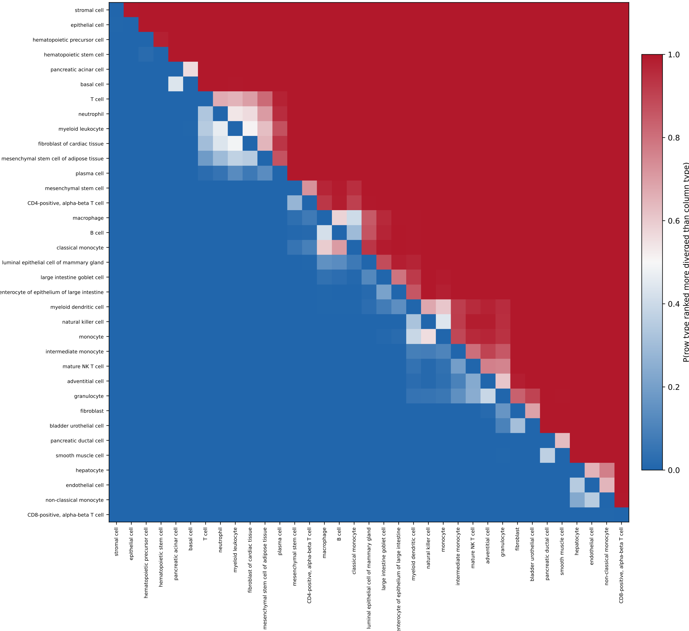
Pairwise Rank-Swap Probability Matrix (n = 1000 bootstrap iterations)
