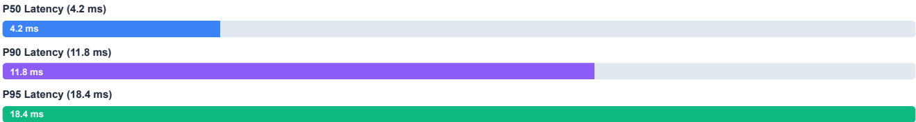
FIGURE 6: EVALUATION OVERHEAD LATENCY DISTRIBUTION PROFILE (MS)
