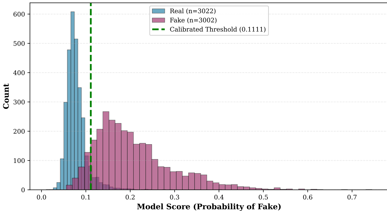
Score Distribution by True Label (v5 Model on Test Set)
