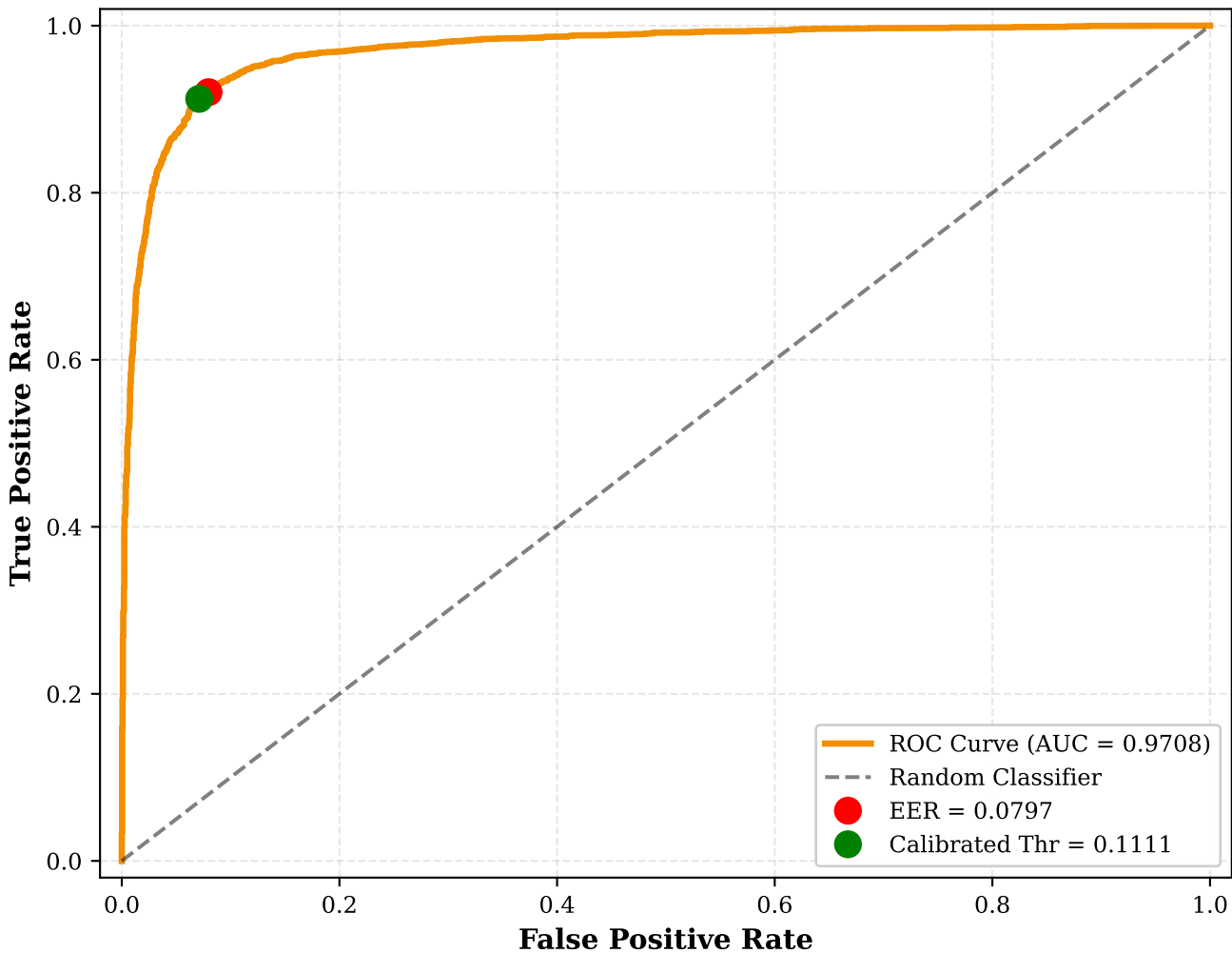
ROC Curve (v5 Model on Test Set)
