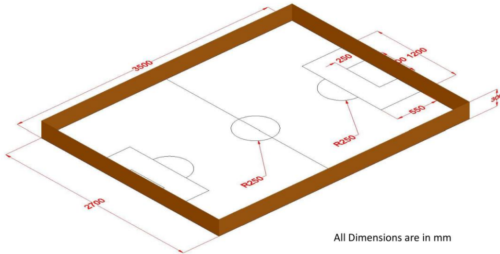
Figure: Official football game arena layout (all dimensions are in millimetres).
