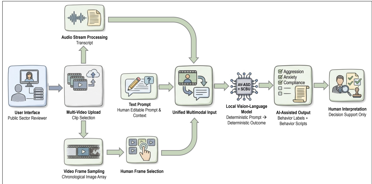
Fig. 2 – System Workflow
