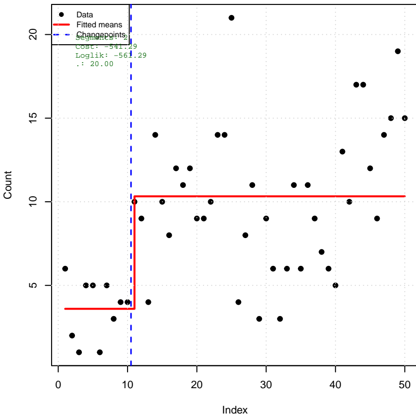
\lambda = 20.0 (2 segments)
