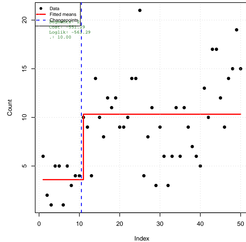
\lambda = 10.0 (2 segments)
