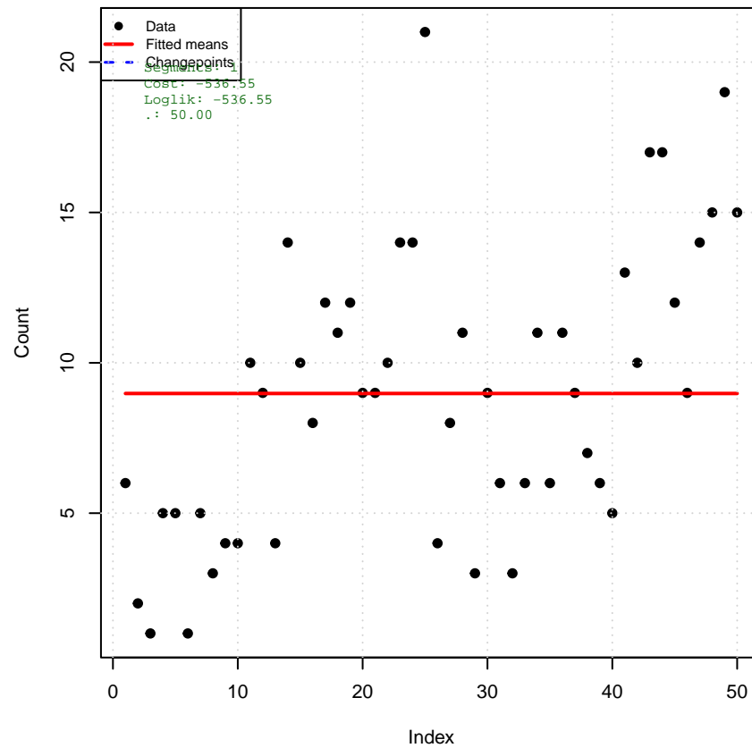
\lambda = 50.0 (1 segments)
