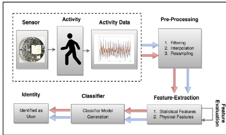
Figure 1: The ActID Framework.
