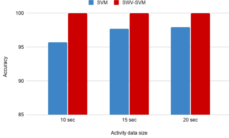
Figure 13: Impact of activity data size.
