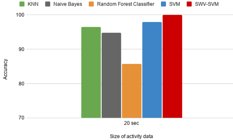
Figure 11: Performance comparison between SWV classifier and other traditional classifiers.
