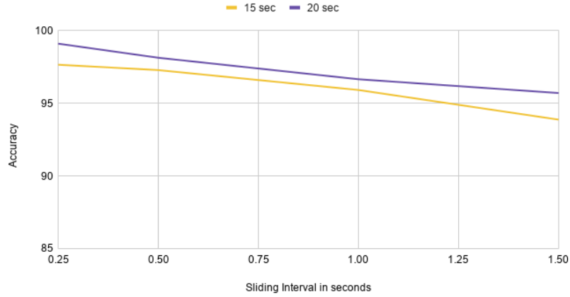
Figure 9: Impact of sliding interval.
