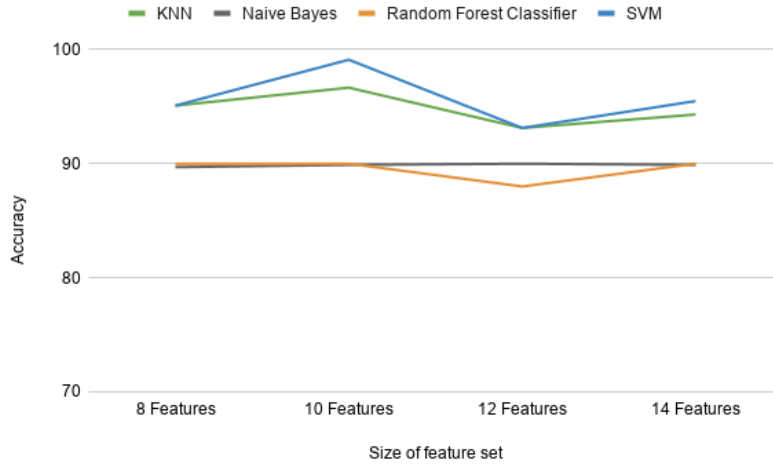
Figure 10: Impact of number of features.
