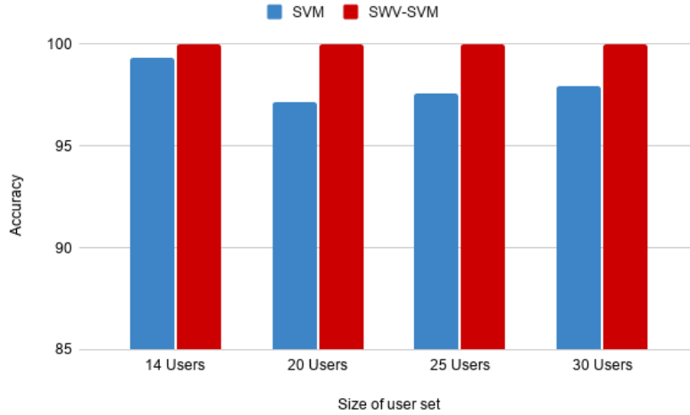
Figure 12: Scalability of SWV.
