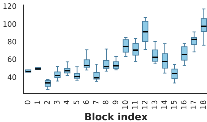
Target projection norm
