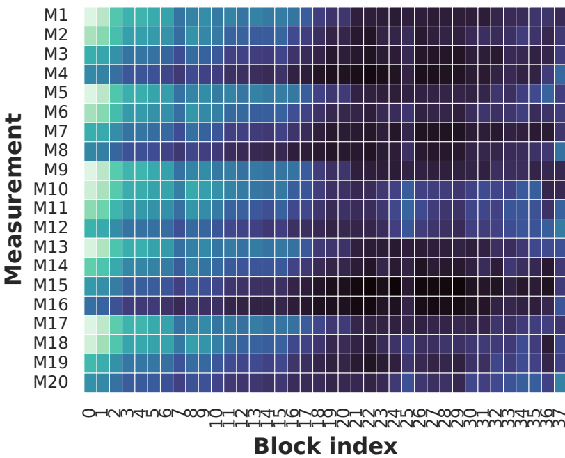
Celebrities
