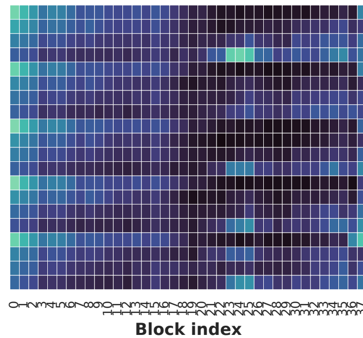
Objects
