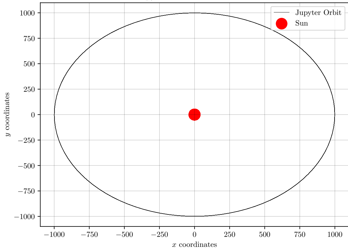
Jupyter Orbit around the sun
