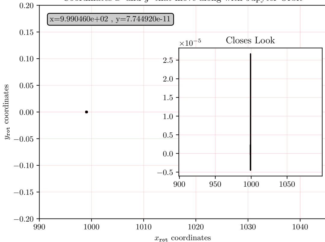
Coordinates x' and y' that move along with Jupyter Orbit
