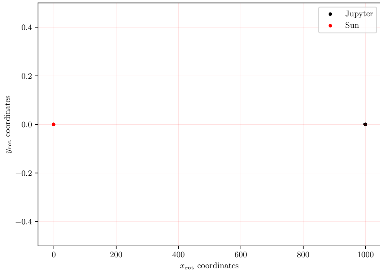
Coordinates x' and y' that move along with Jupyter Orbit
