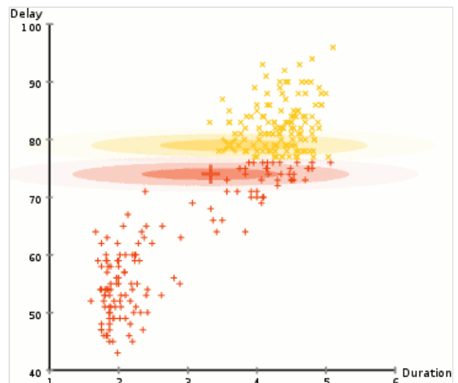
Expectation–maximisation clustering of Old Faithful eruption data starts from a random guess but then successfully converges on an accurate clustering of the two physically distinct modes of eruption.
