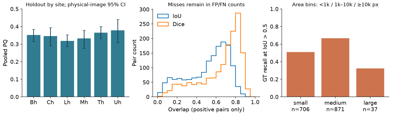
Figure 3: Protected holdout diagnostics. Left: site-wise pooled PQ and physical-image bootstrap intervals. Middle: positive-pair overlap distributions; missing objects remain in FP/FN counts. Right: GT recall by native mask area, showing size-dependent misses.
