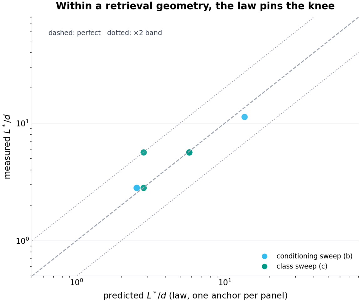
Figure 7: Measured knees vs the law’s ratio predictions (log-log), one anchor point per retrieval geometry. Six of seven points fall within 11% of the diagonal; the seventh is the class-mismatch case whose bias term the law absorbs.
