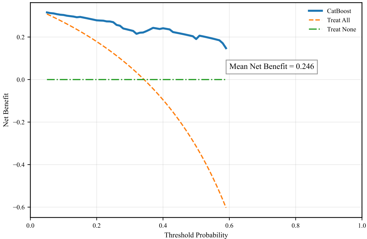
Decision Curve Analysis
