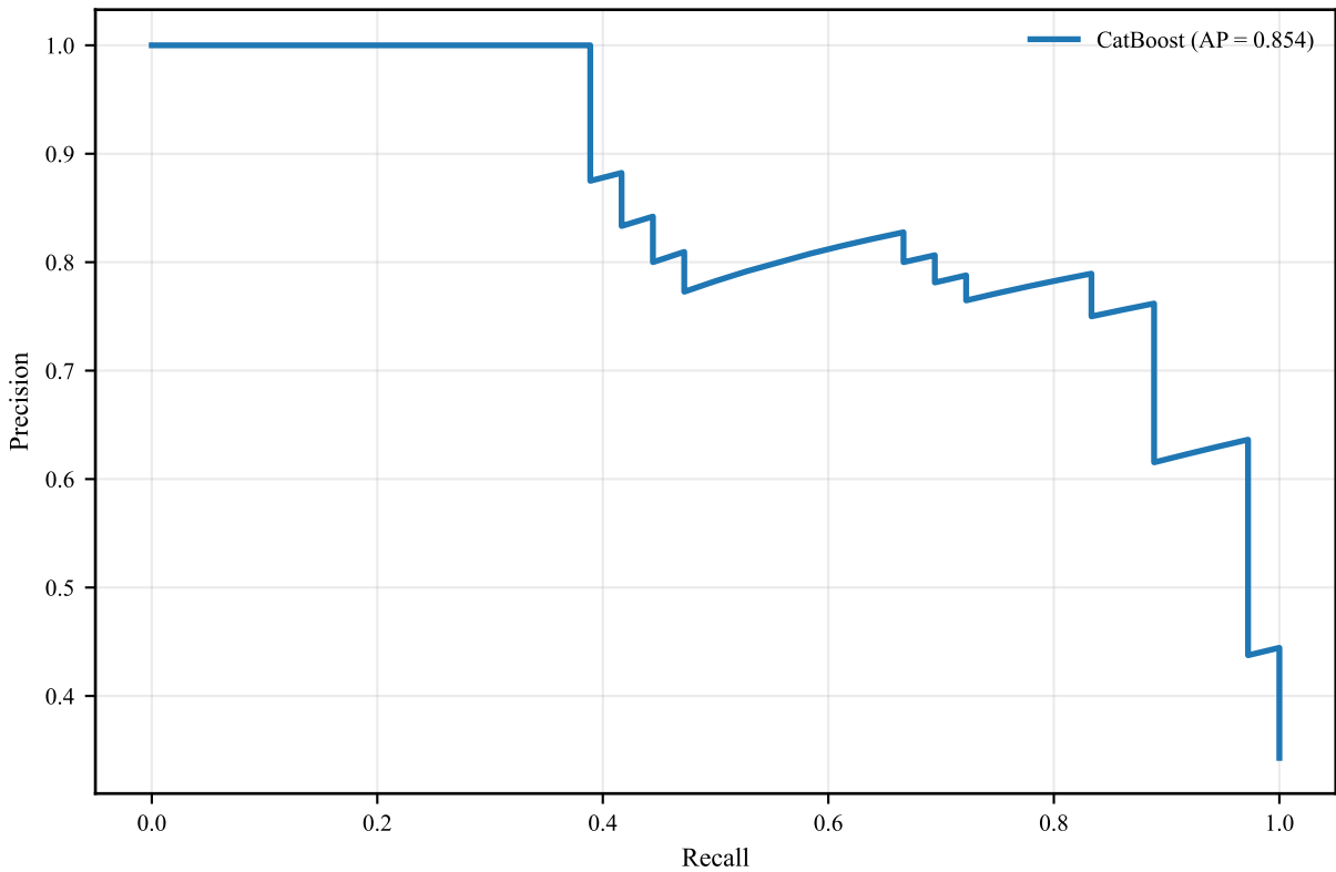
Precision-Recall Curve
