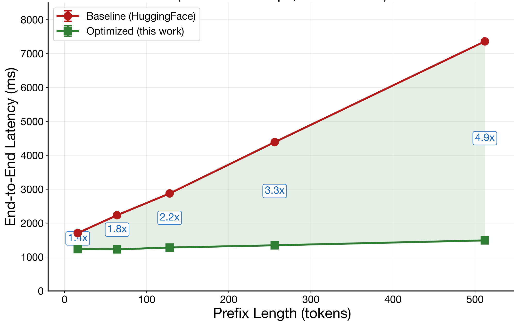
Latency vs. Prefix Length (50 diffusion steps, C4 validation)
