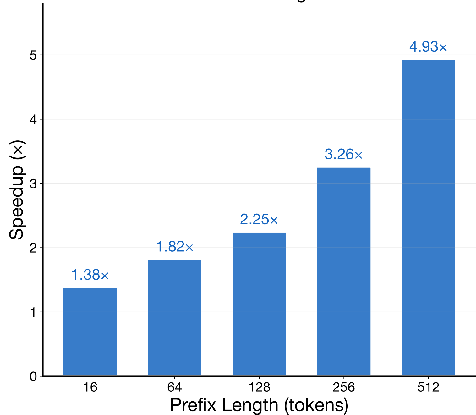
Speedup Scales with Context Length
