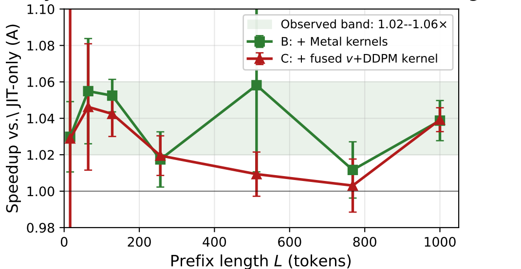
Systems wins are constant in L , \sim 1.04\times on average
