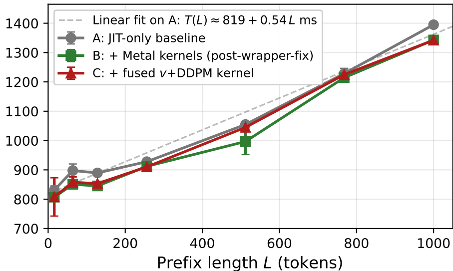
Wall time scales linearly with prefix length
