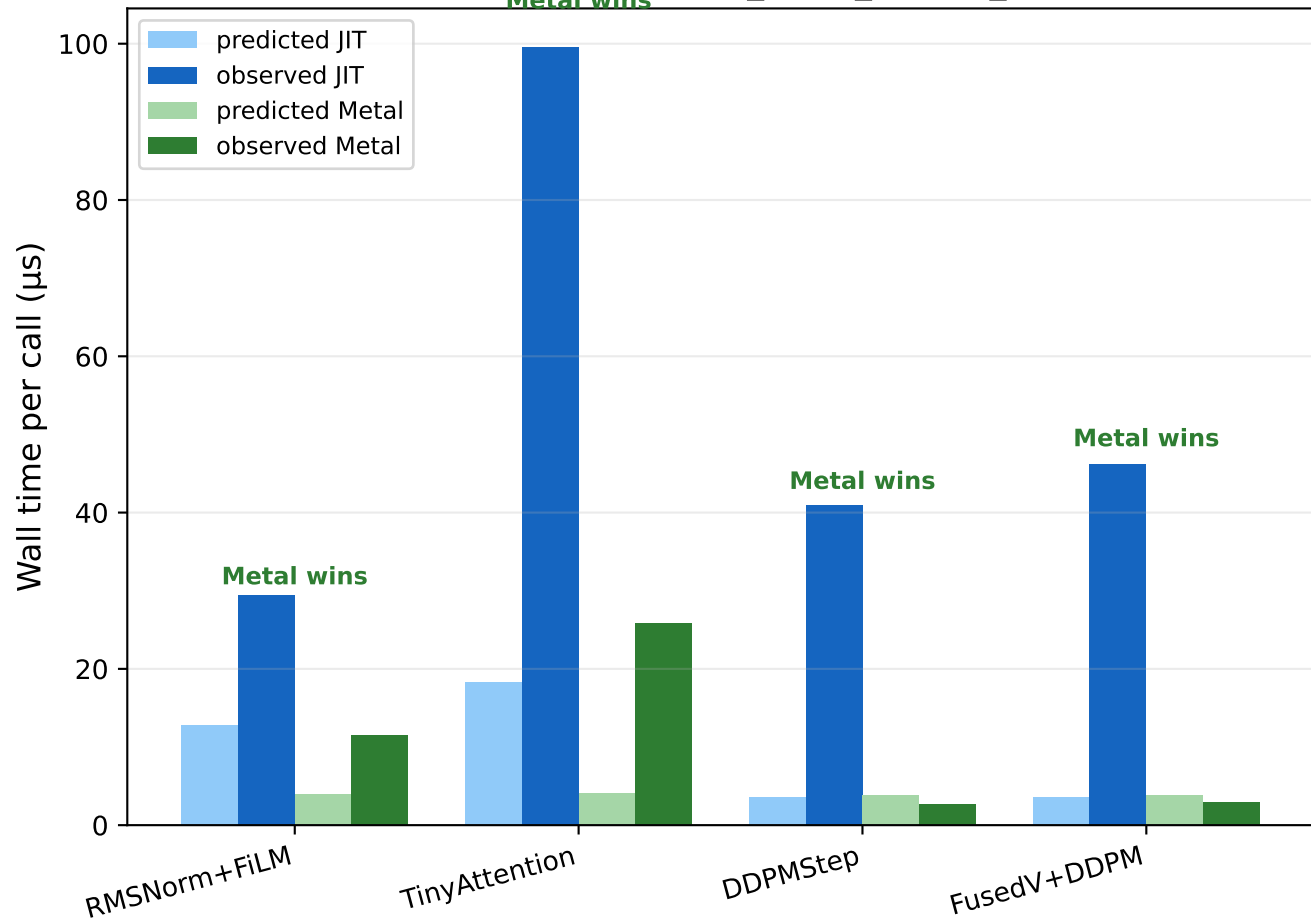
Crossover model: predictions vs observations (✓ Metal wins where K_{\text{eff}} \cdot T_{\text{jit}} > T_{\text{metal}} )
