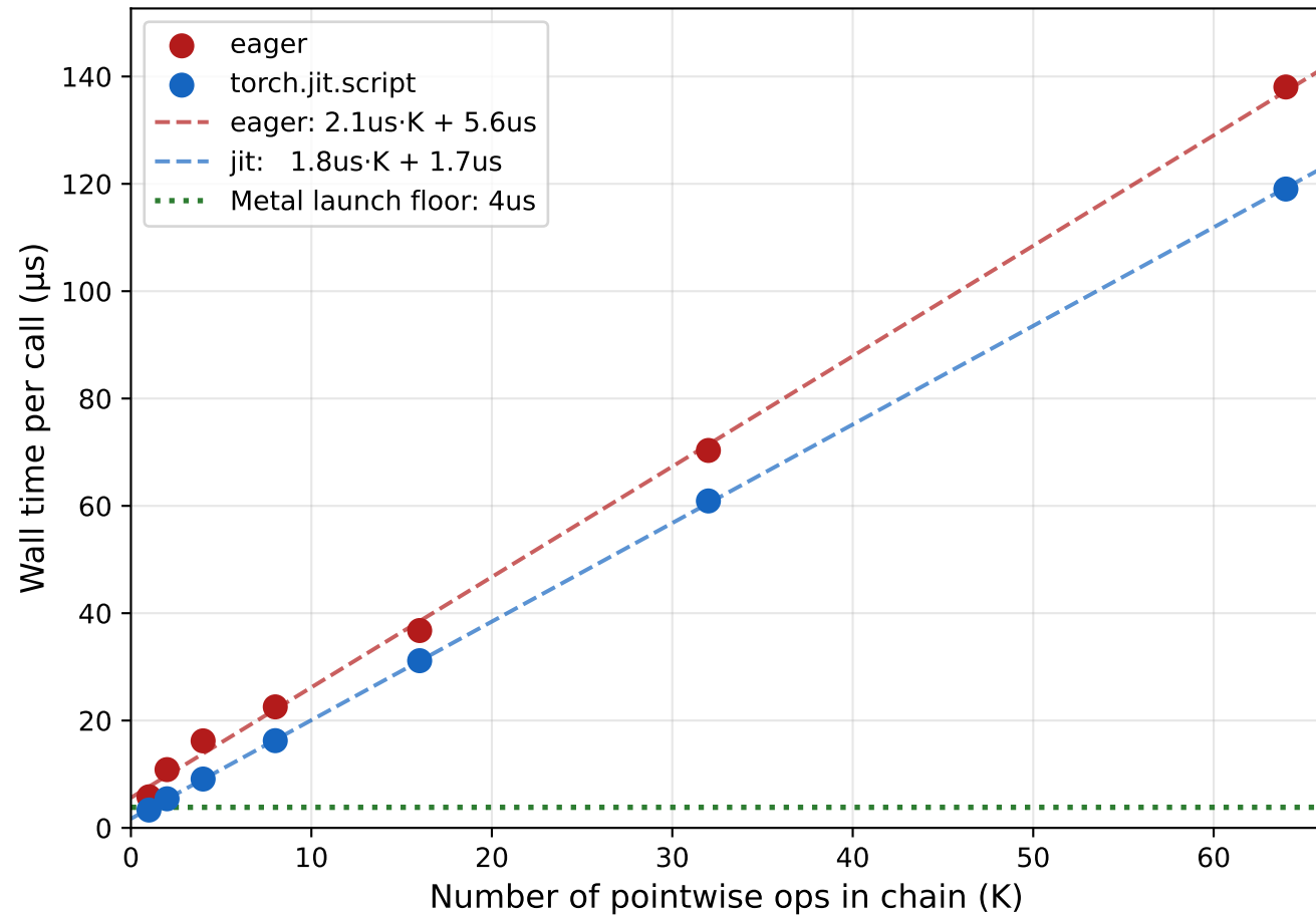
M4 Max dispatch-cost calibration (D=768 floats, B=1)
