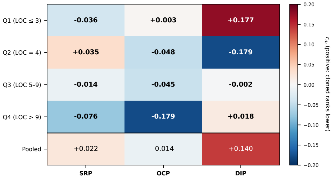
Size-stratified rank-biserial within method-LOC quartiles
