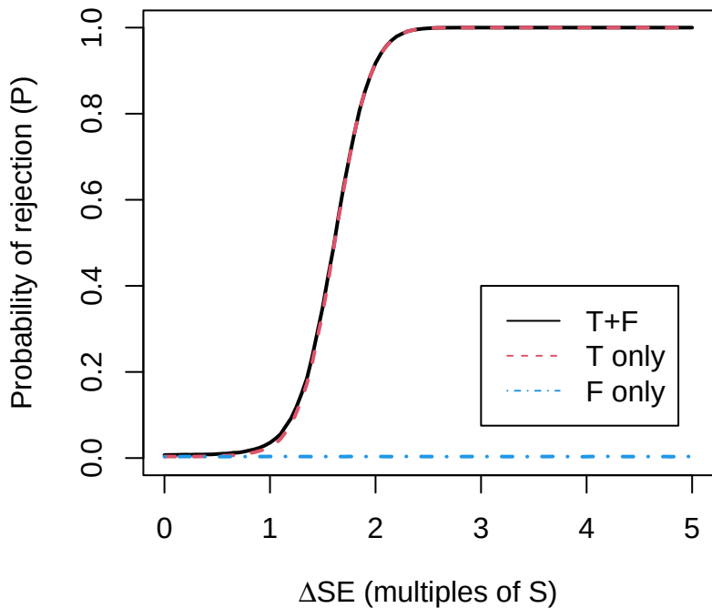
T and F test Bias (50-plex, P=5 \times 10^{-5} )
