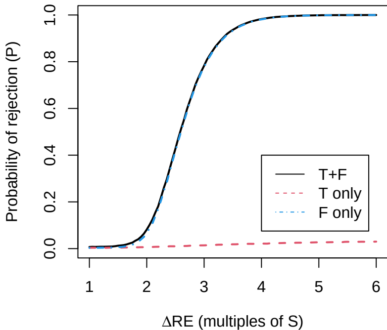
T and F test Imprecision (50-plex, P=5 \times 10^{-5} )
