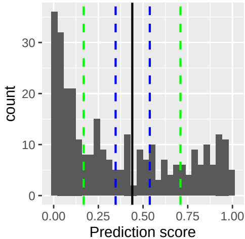
XGBoost
