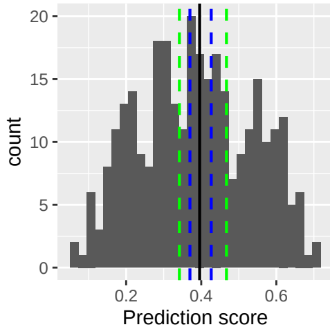
Random Forest
