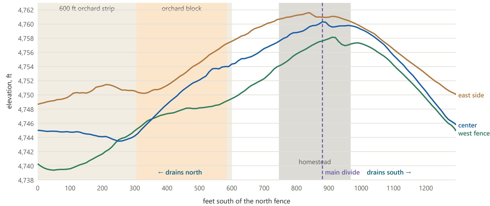
Spot elevations in feet, every 100 ft south of the north fence
