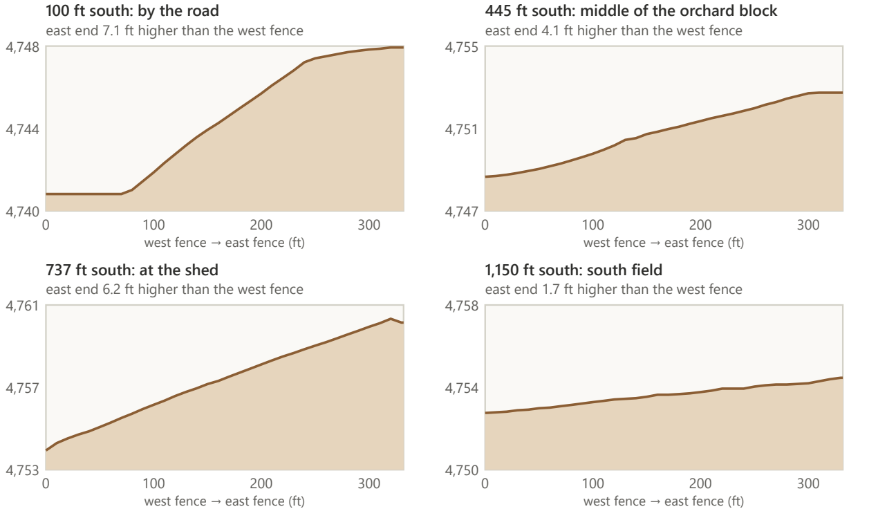
East–west cross-sections (vertical scale exaggerated)
