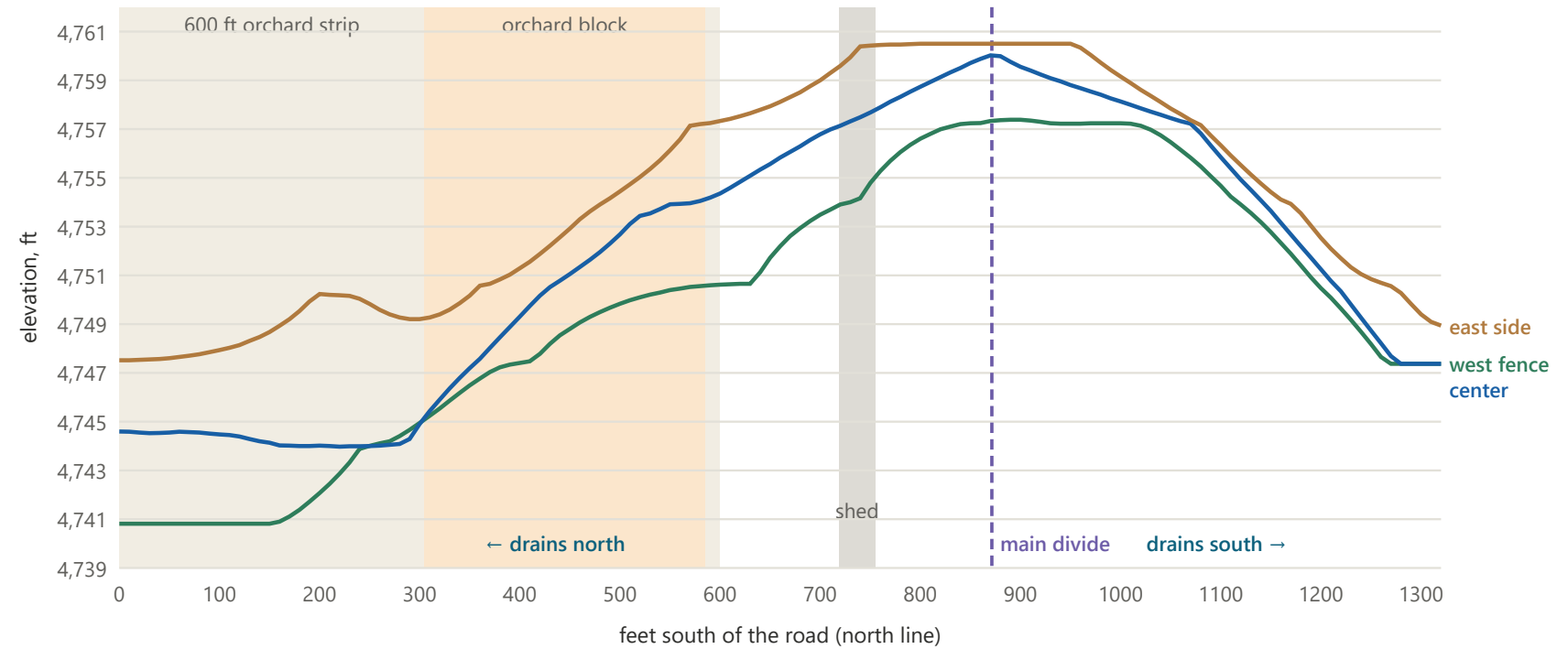
Spot elevations in feet, every 100 ft south of the road
