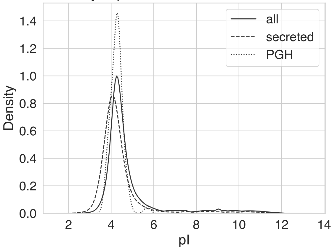
Density of pI from GTDB class Halobacteria
