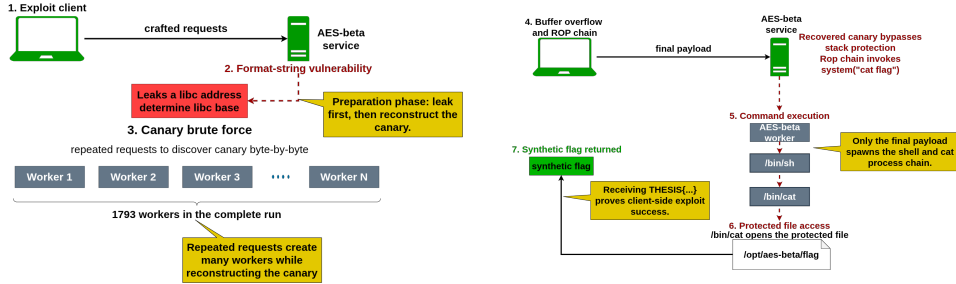
Figure 6.3: Controlled AES-beta exploitation flow. The preparation phase is shown on the left, while the final payload and resulting process chain are shown on the right. Shell execution, cat execution and flag access satisfy the configured four-event detector sequence.
