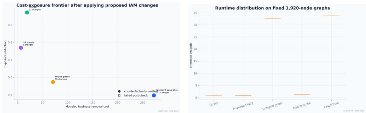
(a) Registered-instance remediation frontier; Table 2 reports the 15-organization follow-up.
