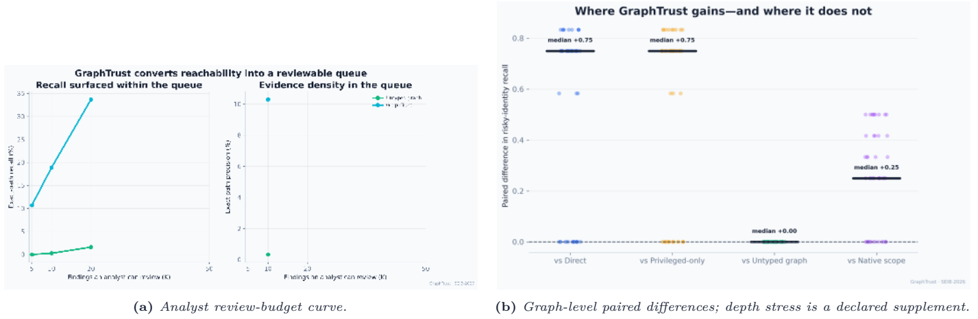
Figure 2: The primary operational endpoint is reviewable evidence, with path-depth results reported separately from the confirmatory aggregate.
