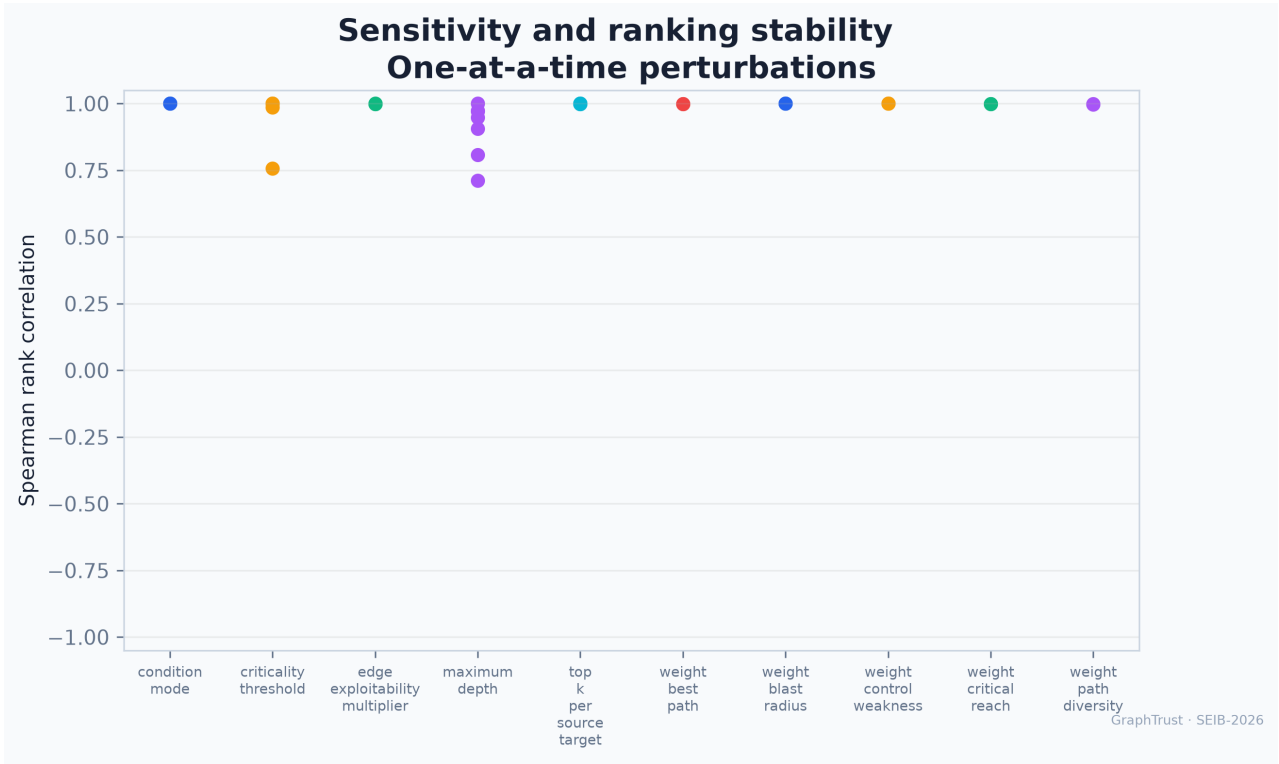
Figure 10: One-at-a-time and 1,000-sample weight sensitivity.
