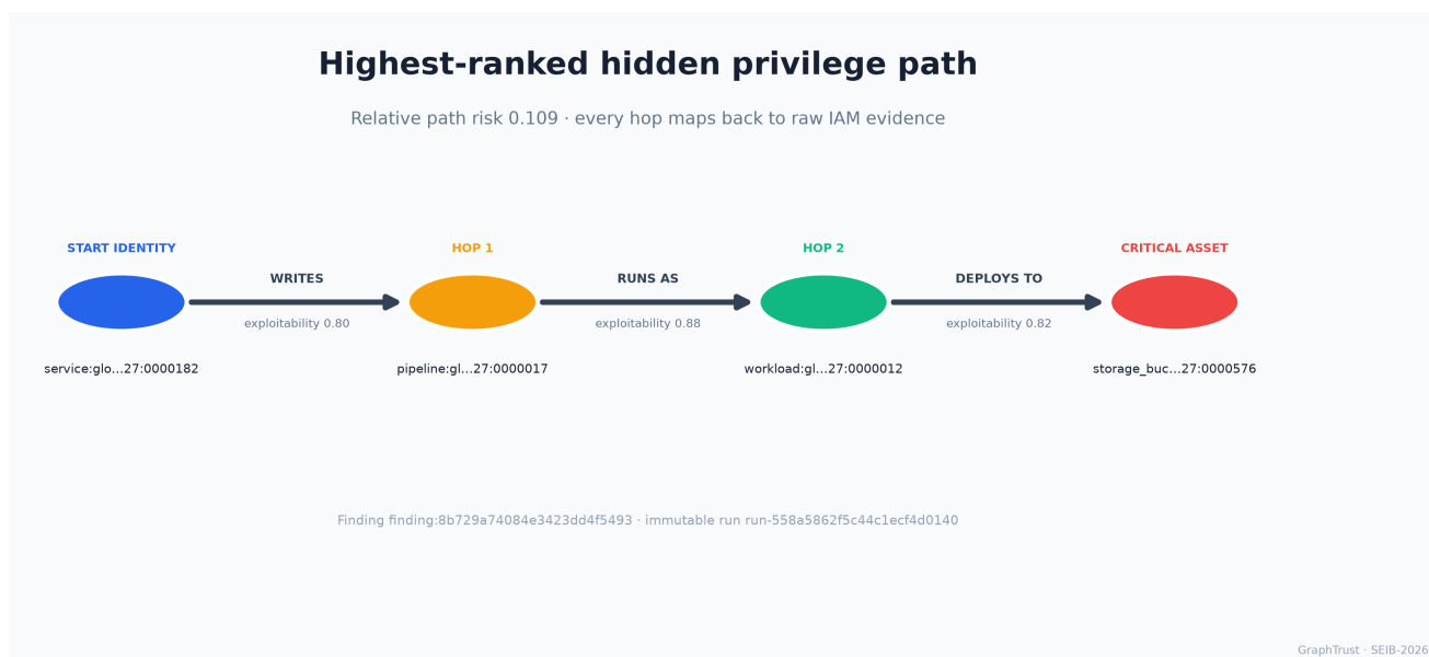
Figure 3: Highest-ranked evidence-linked privilege path.
