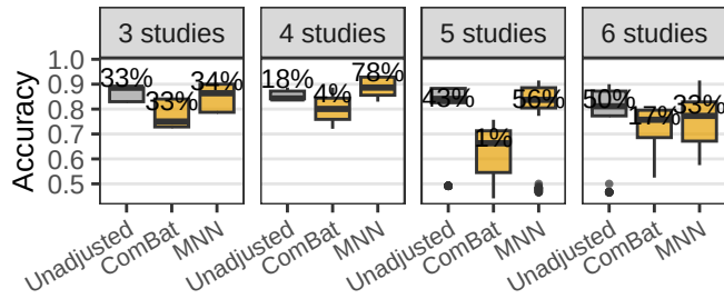
Adjuster Effectiveness – LightGBM
