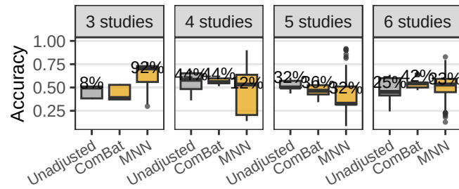
Adjuster Effectiveness – Random Forest
