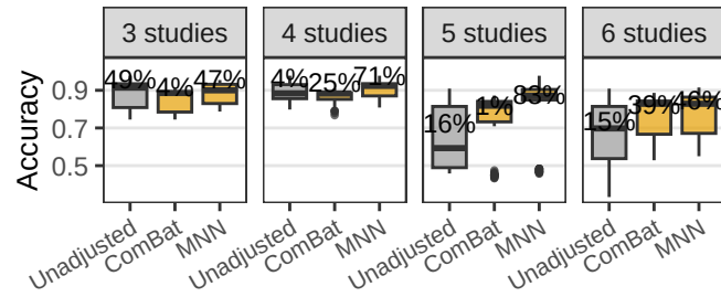
Adjuster Effectiveness – XGBoost
