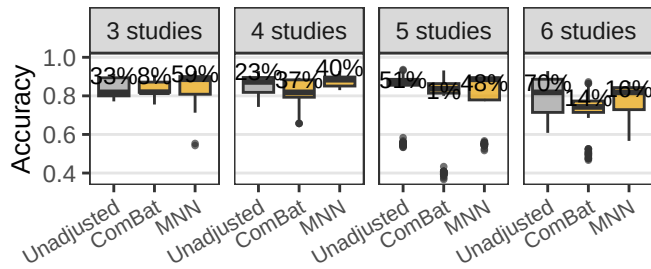
Adjuster Effectiveness – KNN
