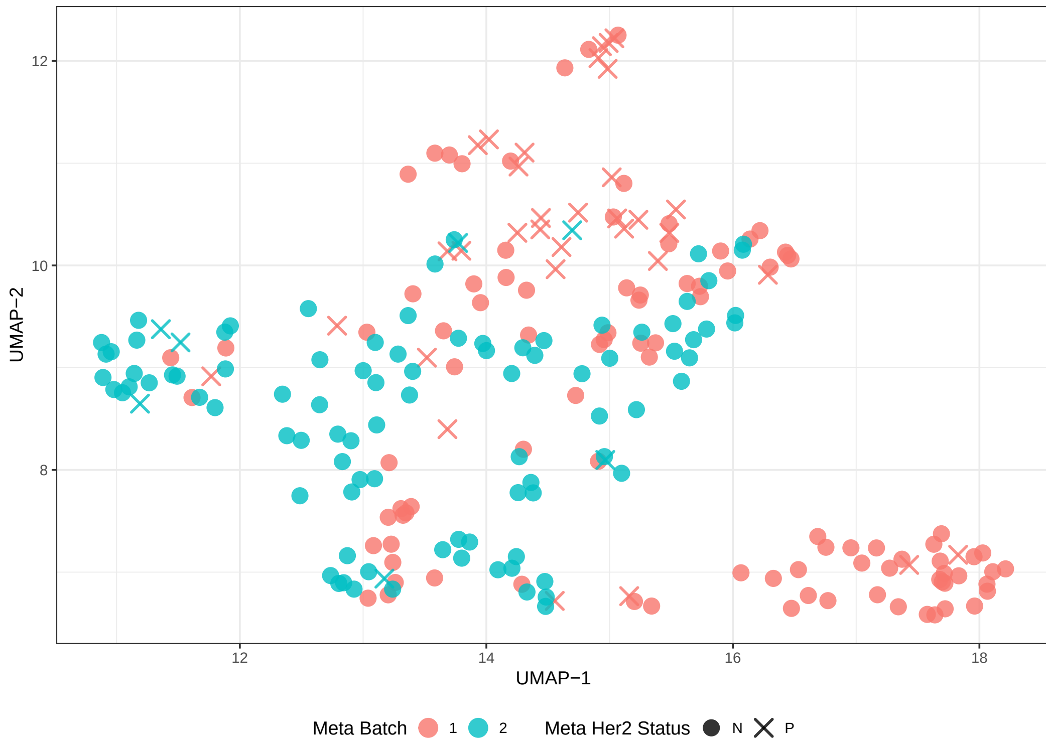
GSE 20194 HER2 – Quantile (UMAP) Colored by Meta Batch , Shaped by Meta Her2 Status
