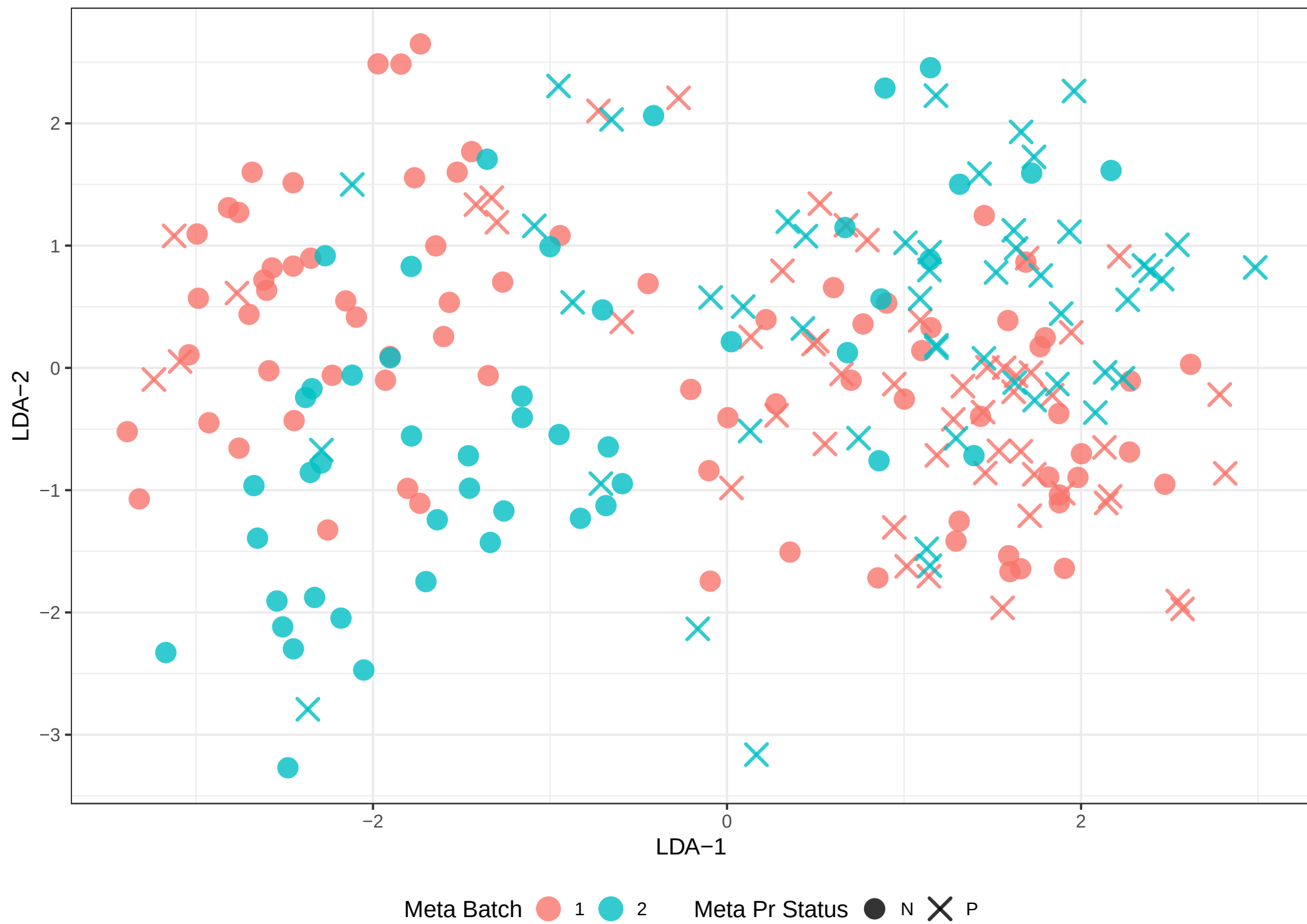
GSE 20194 PR – Wasserstein (LDA) Colored by Meta Batch , Shaped by Meta Pr Status
