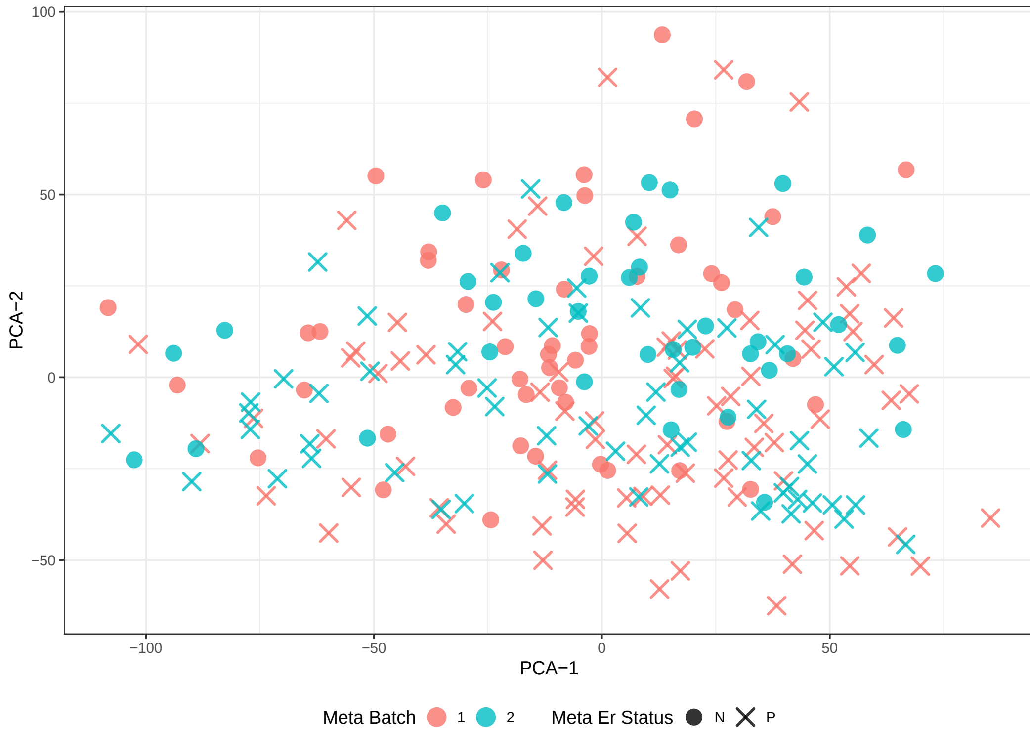
GSE 20194 ER – Seurat_scaling (PCA) Colored by Meta Batch , Shaped by Meta Er Status
