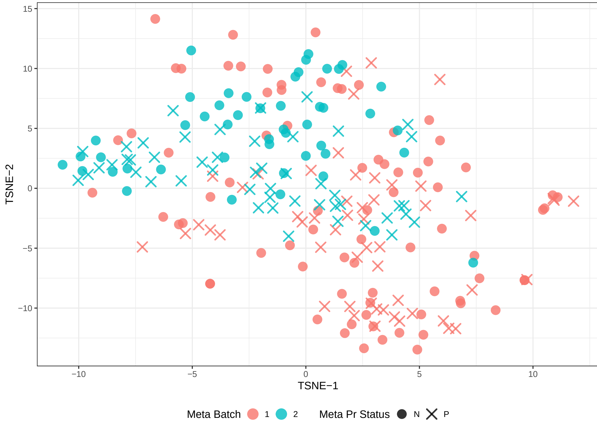
GSE 20194 PR- Quantile (TSNE) Colored by Meta Batch , Shaped by Meta Pr Status
