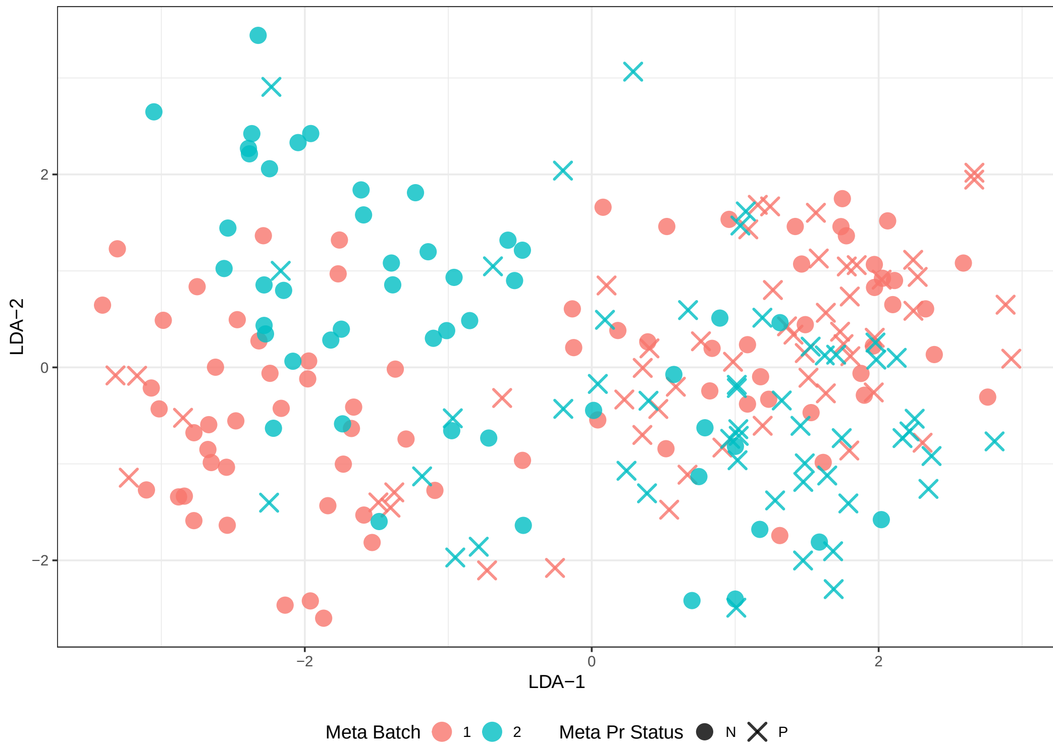
GSE 20194 PR – Combat_target (LDA) Colored by Meta Batch , Shaped by Meta Pr Status
