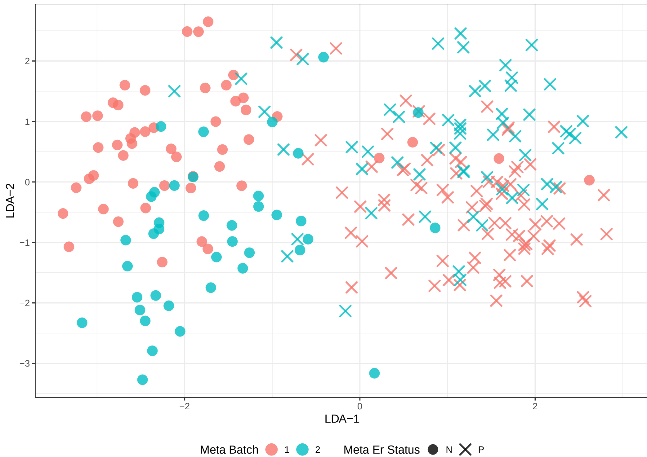
GSE 20194 ER – Wasserstein (LDA) Colored by Meta Batch , Shaped by Meta Er Status
