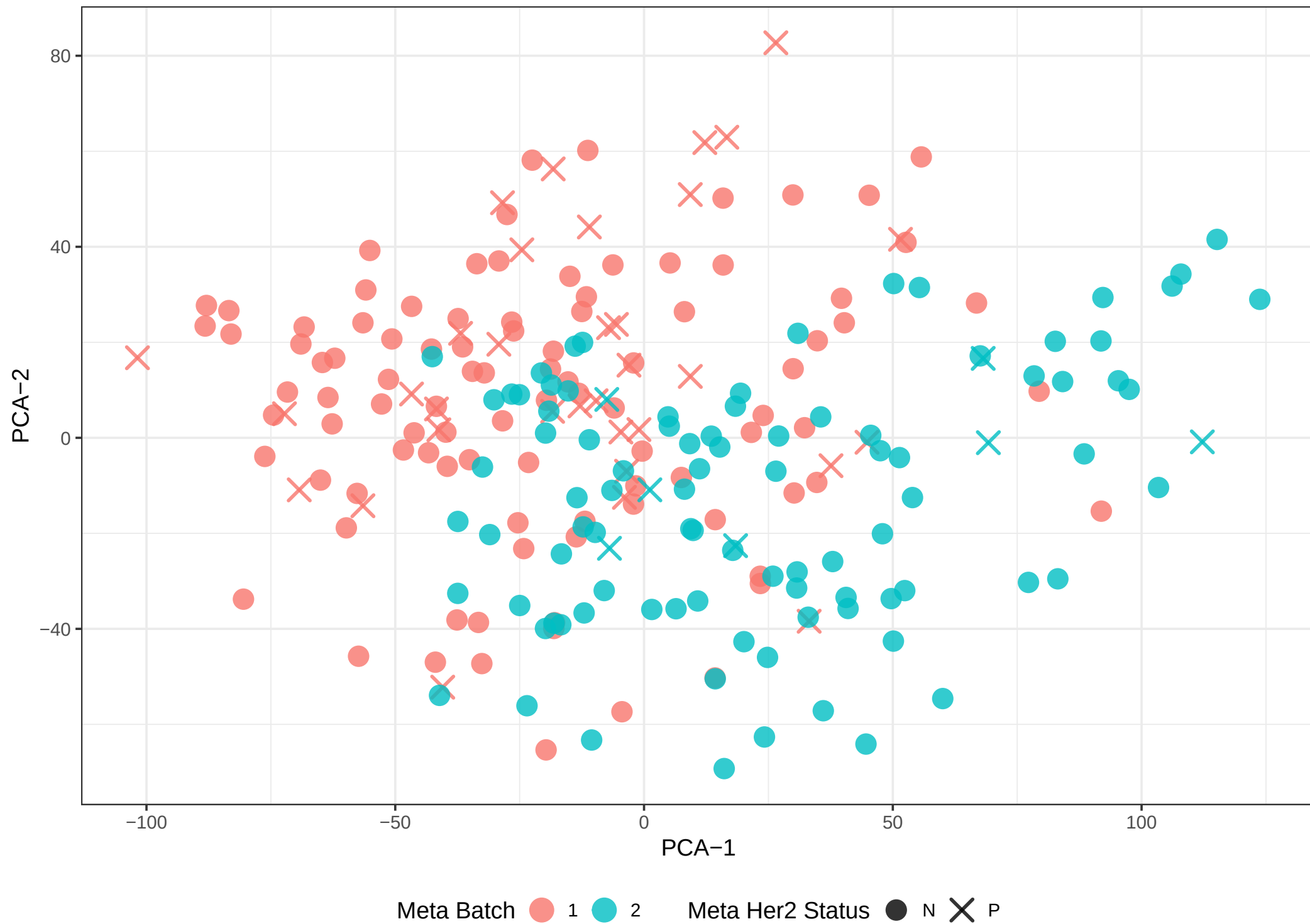
GSE 20194 HER2 – Harmony (PCA) Colored by Meta Batch , Shaped by Meta Her2 Status
