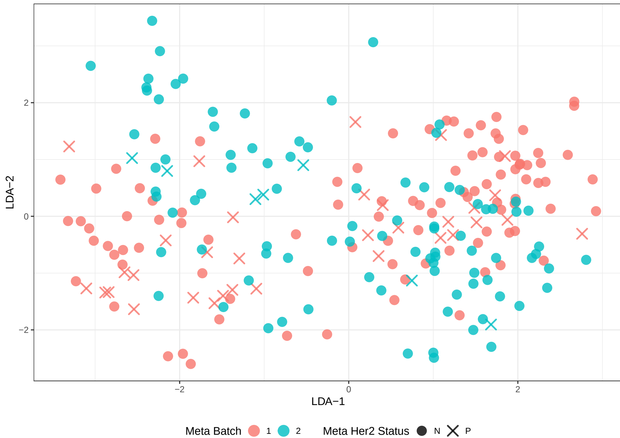
GSE 20194 HER2 – Combat_target (LDA) Colored by Meta Batch , Shaped by Meta Her2 Status
