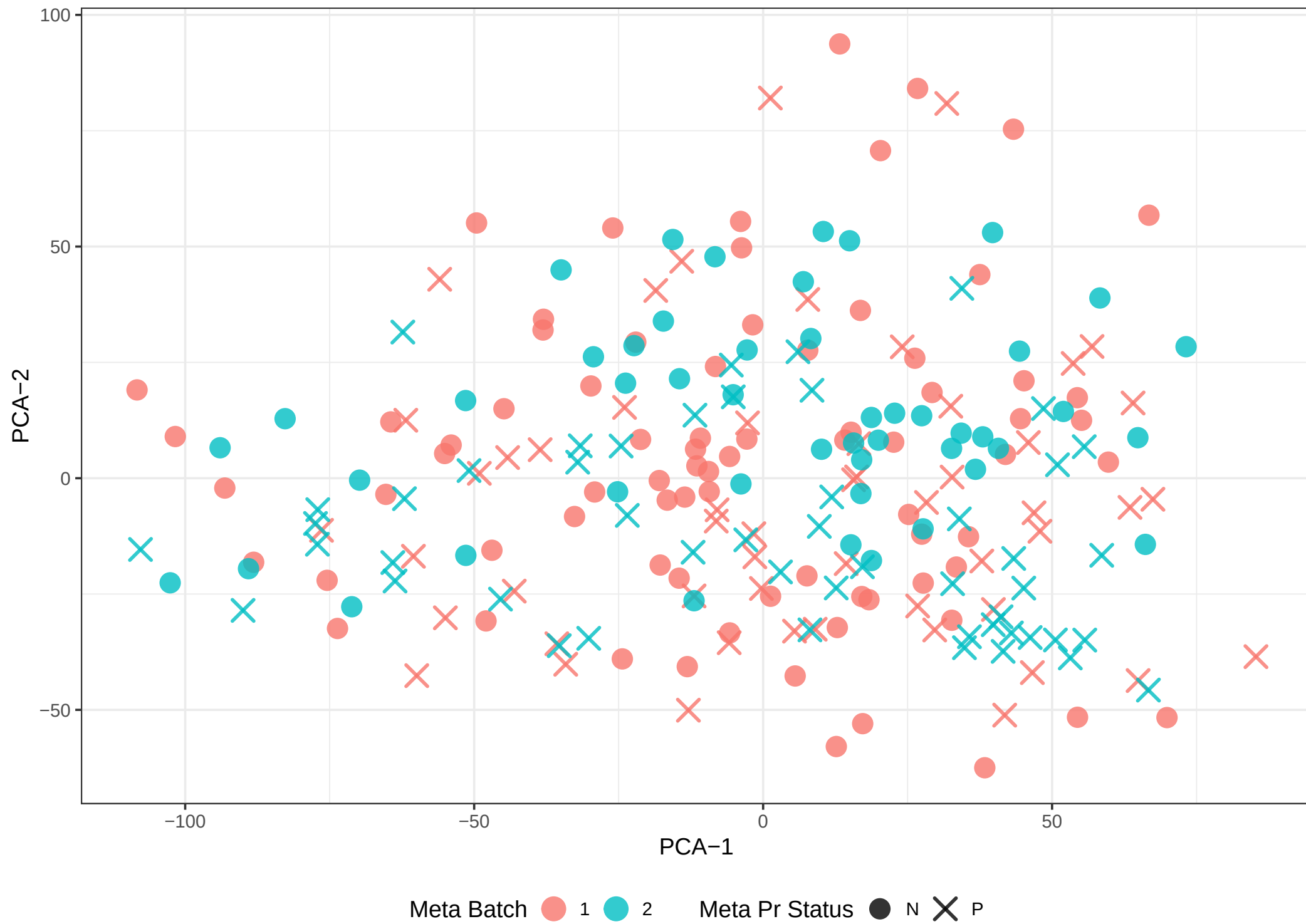
GSE 20194 PR – Seurat_scaling (PCA) Colored by Meta Batch , Shaped by Meta Pr Status
