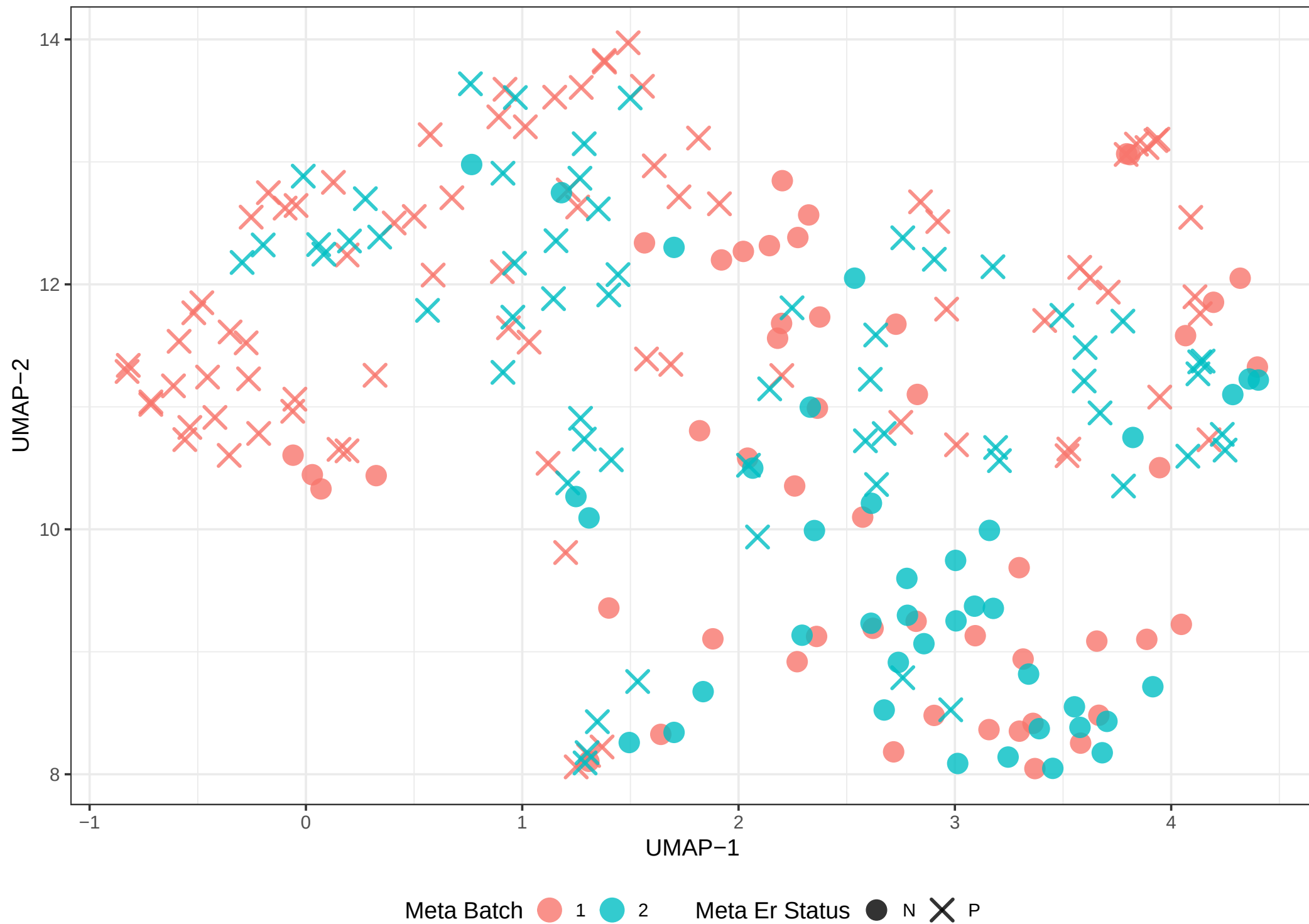
GSE 20194 ER – fastMNN (UMAP) Colored by Meta Batch , Shaped by Meta Er Status
