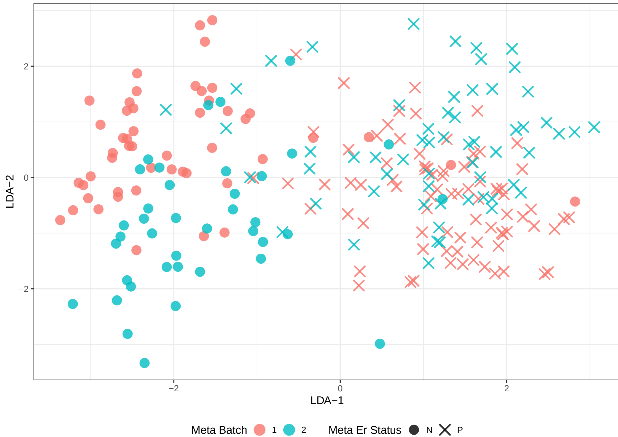
GSE 20194 ER – Npn (LDA) Colored by Meta Batch , Shaped by Meta Er Status
