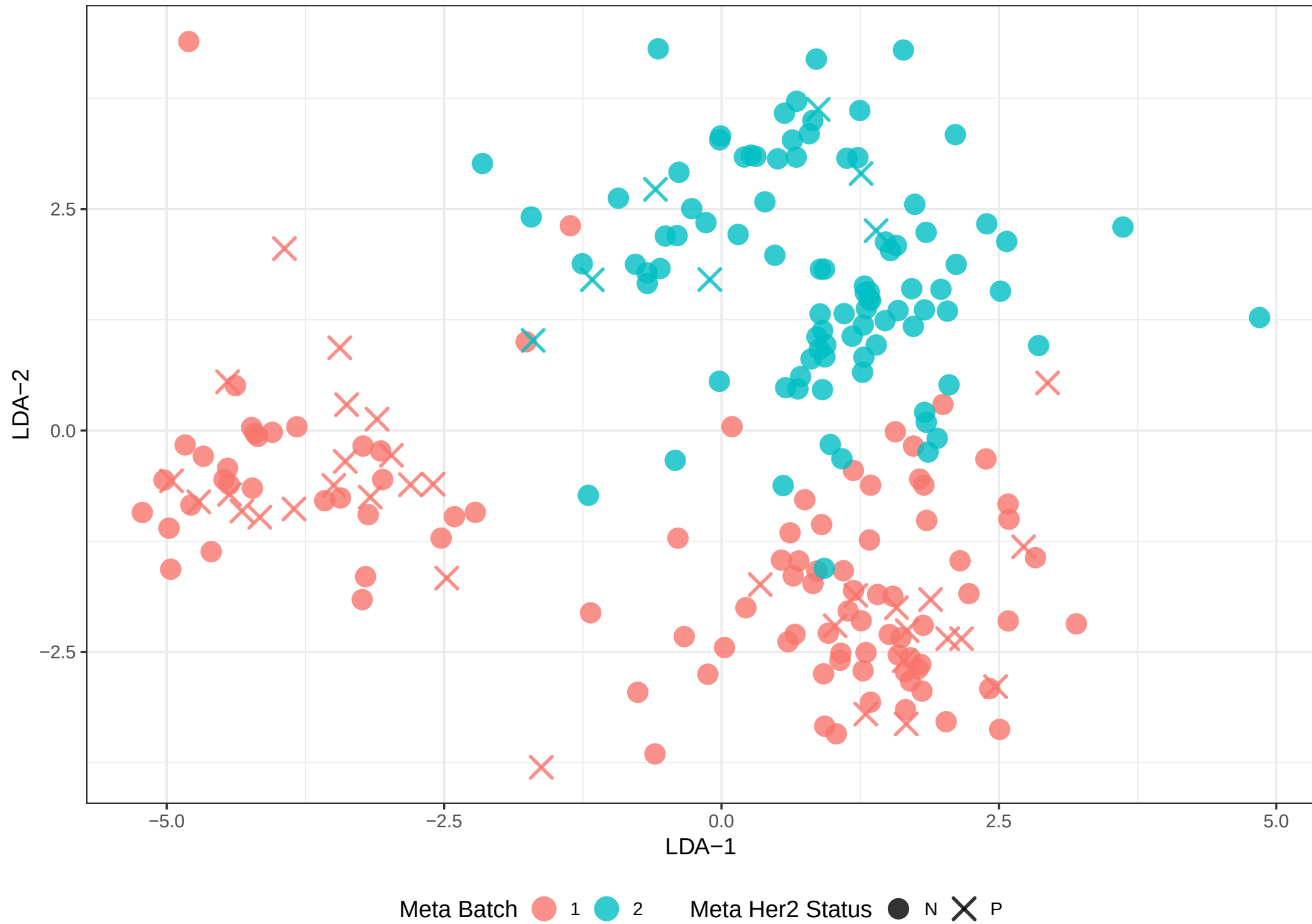
GSE 20194 HER2 – lcvae (LDA) Colored by Meta Batch , Shaped by Meta Her2 Status
