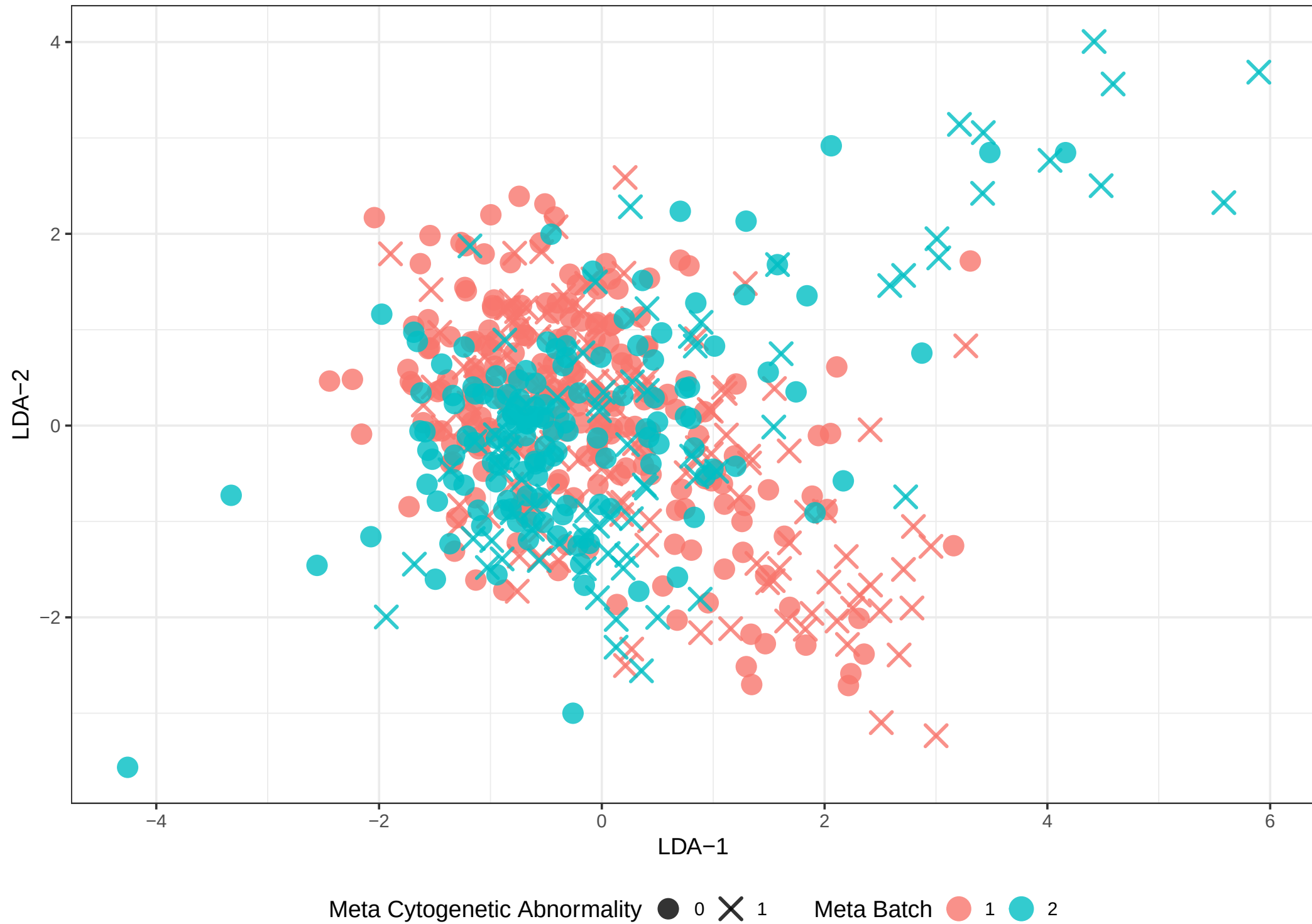
GSE 24080 Cytogenetic Abnormality – Limma (LDA) Colored by Meta Batch , Shaped by Meta Cytogenetic Abnormality
