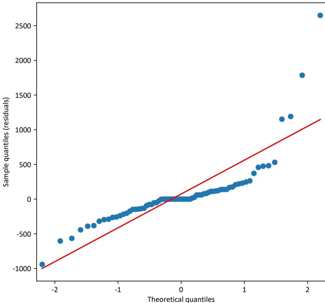
C1_Combined_ALK Robust_Linear_Regression @ 1.5° Residual Q-Q plot (n=71 eyes)
