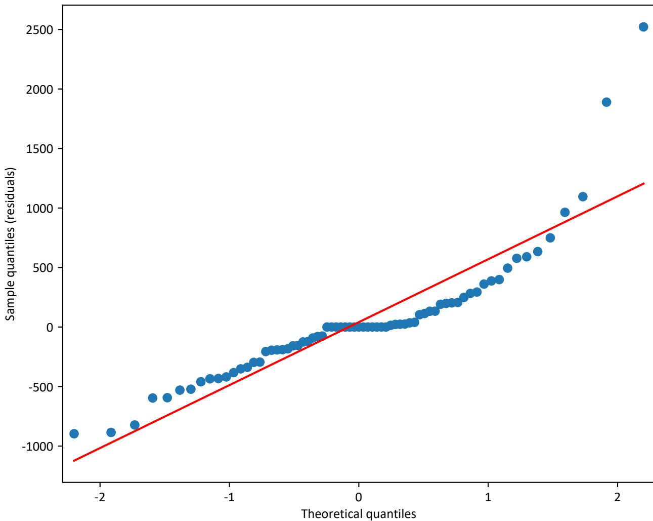
C1_Combined_ALK Lasso @ 1.5 mm Residual Q-Q plot (n=71 eyes)
